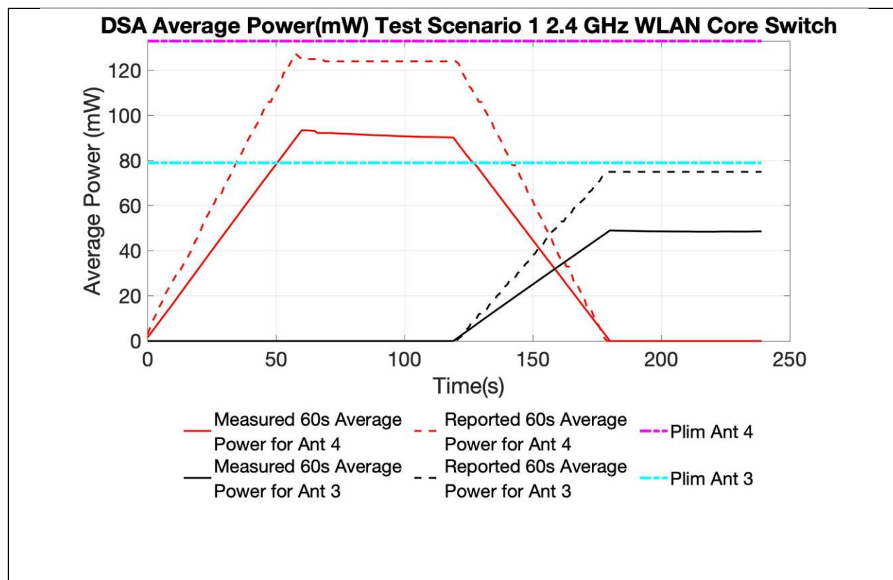
Figure 2 60 Second Average Power vs Time, 2.4GHz
