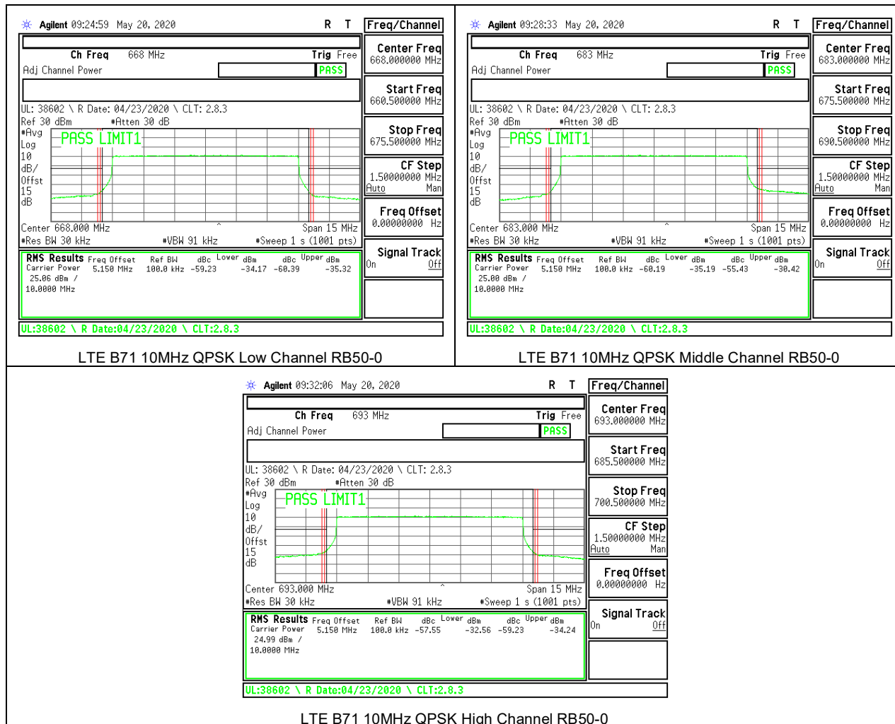
LTE B71 10MHz QPSK High Channel RB50-0
