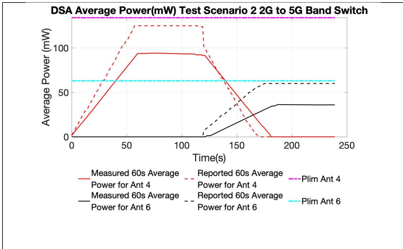
Figure 8 60 Second Average Power vs Time during Band Switch
