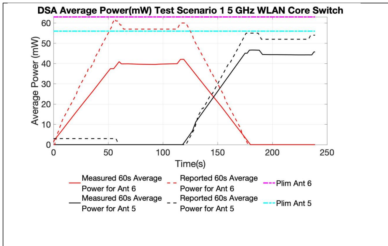
Figure 5 60 Second Average Power vs Time, 5GHz
