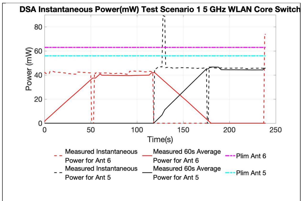
Figure 6 60 Second Average Power vs Time and Instantaneous Power, 5GHz
