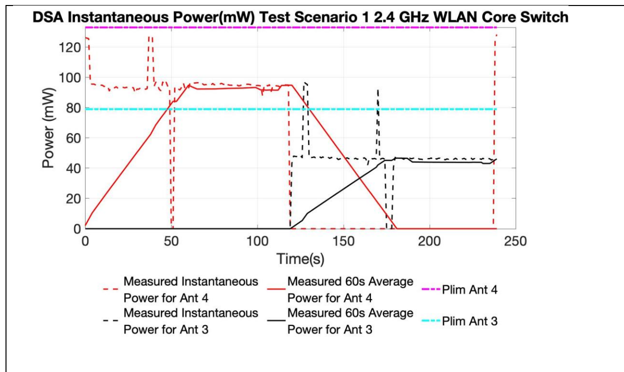
Figure 3 60 Second Average Power vs Time and Instantaneous Power, 2.4GHz
