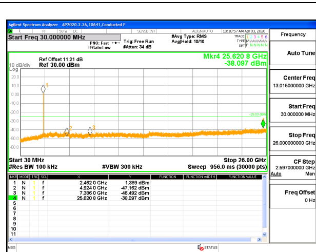
OUT-OF-BAND HIGH CHANNEL 11 ANT 3
