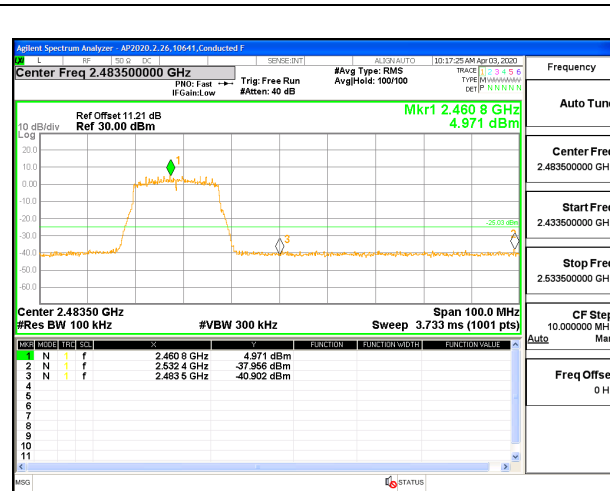
HIGH CHANNEL 11 BANDEDGE ANT 3
