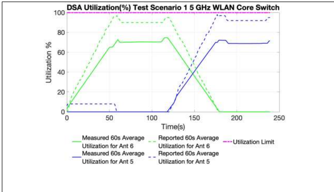
Figure 3 60 Second Aggregated SAR Utilization vs Time, 5GH
