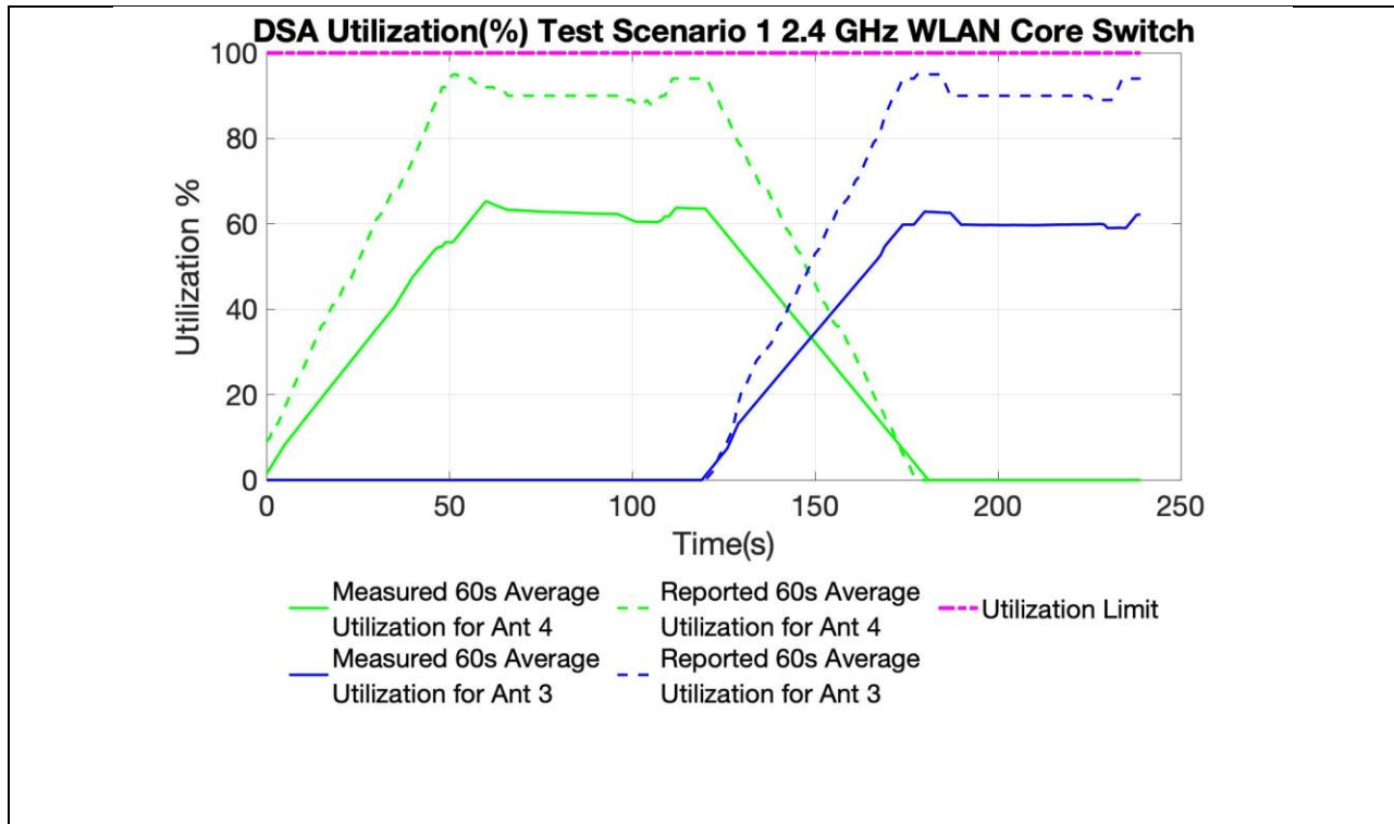
Figure 1 60 Second Aggregated SAR Utilization vs Time, 2.4GHz
