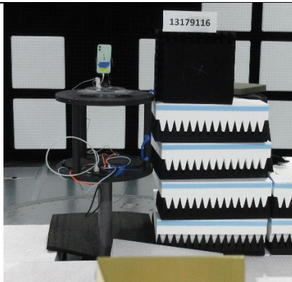
40 – 50 GHz (FRONT)
