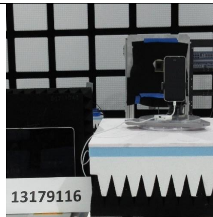
18 - 26 GHz (BACK)
