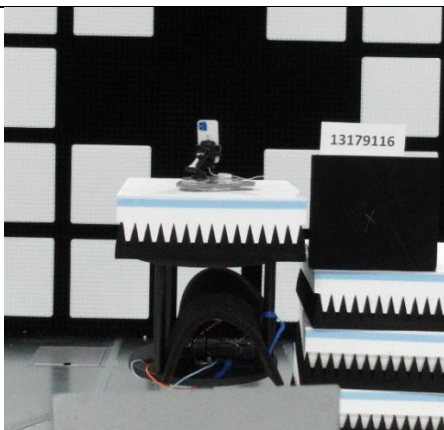
18 - 26 GHz (FRONT)
