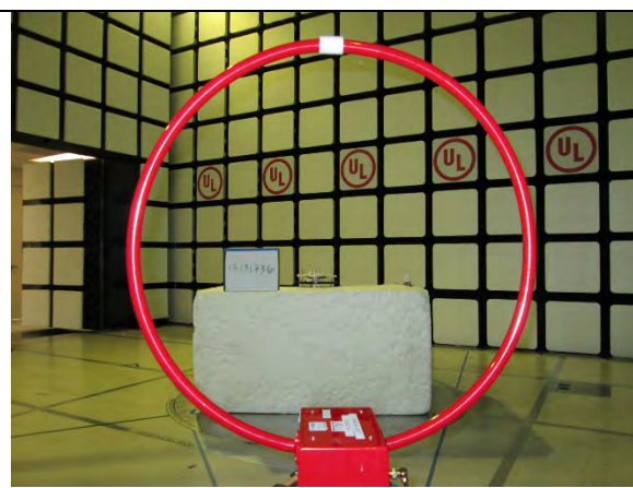
FCC BELOW 30MHz (BACK)
