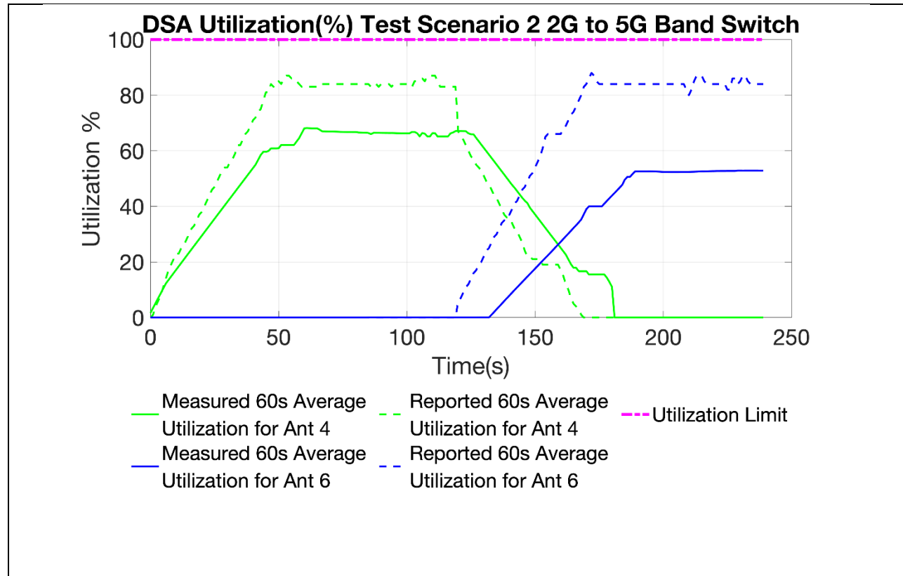
Figure 7 60 Second Aggregated SAR Utilization vs Time during Band Switch
