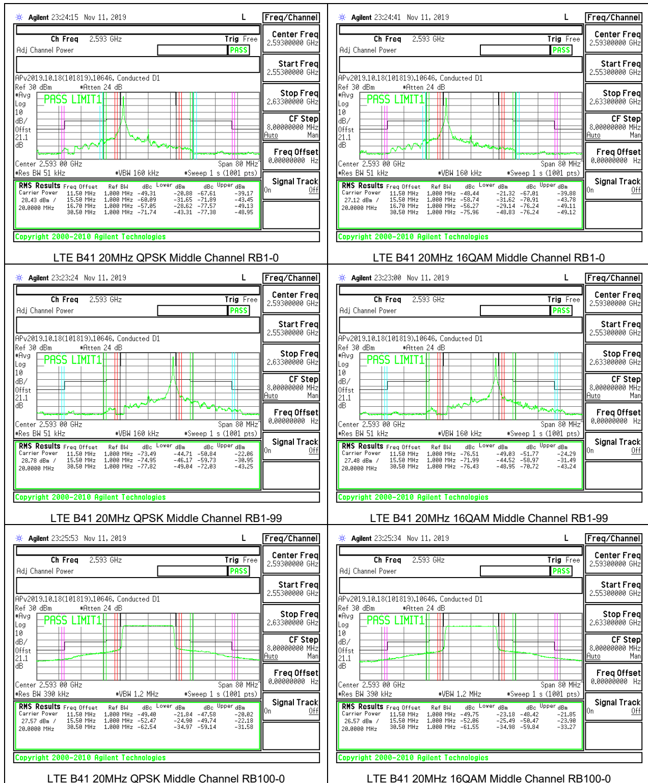
LTE B41 20MHz QPSK Middle Channel RB100-0
