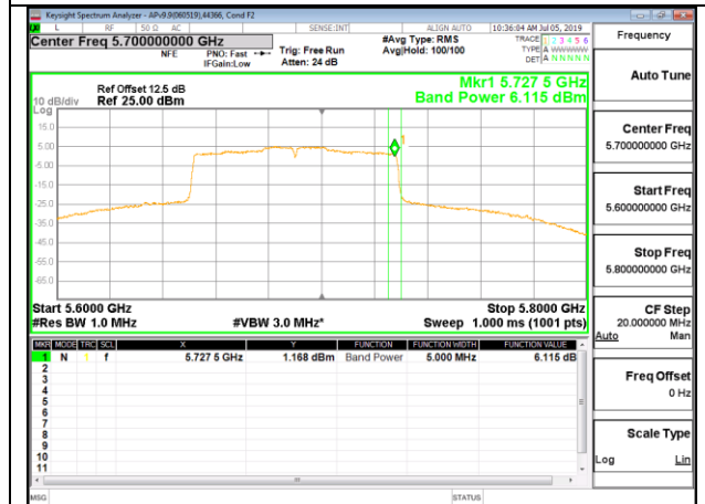
CHANNEL 138 POWER
