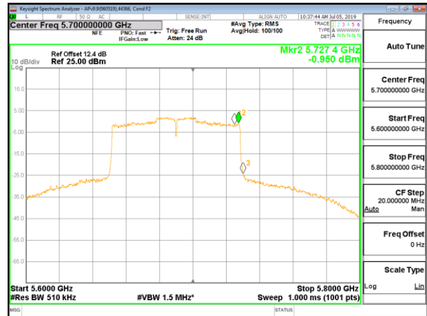
CHANNEL 138 PSD
