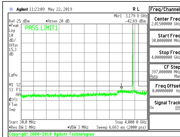
LTE B48 5MHz 16QAM Low Channel RB1-0 ID: 39004
