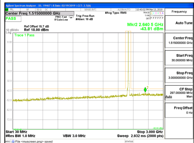
LTE B30 5MHz 16QAM Middle Channel RB1-0
