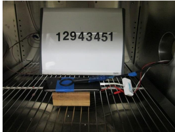
FREQUENCY TOLERANCE
