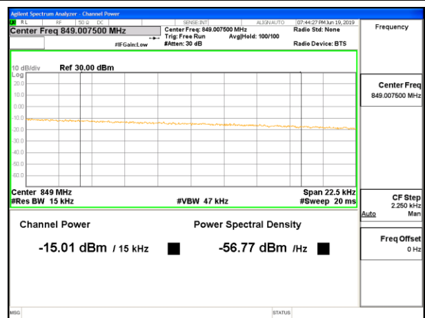
CDMA BC0 1xEV-DO Rev A High Channel (ID:12491)
