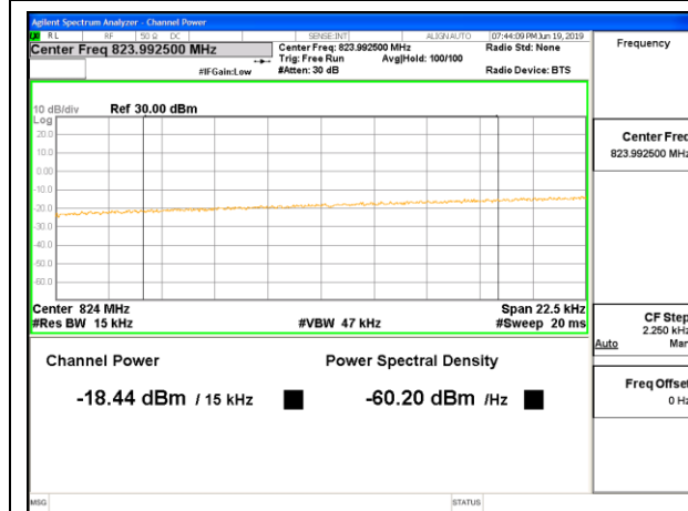
CDMA BC0 1xEV-DO Rev A Low Channel (ID:12491)
