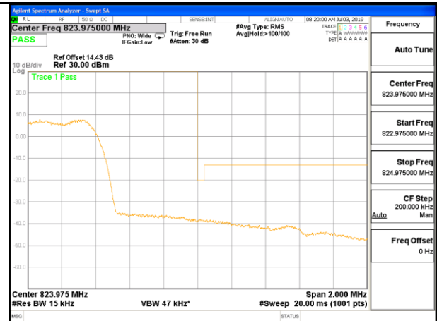
CDMA BC10 1xRTT High Channel, RBW=1% of EBW (ID:12491)
