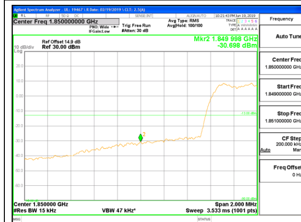
CDMA BC1 1xEV-DO Rev A Low Channel
