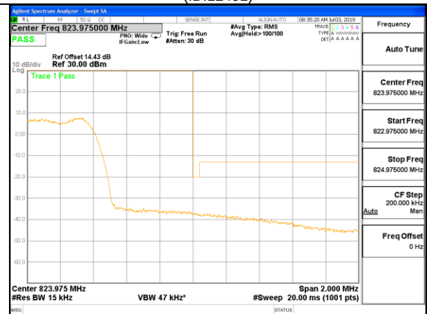
CDMA BC10 1xEV-DO Rev A High Channel, RBW=1% of EBW (ID:12491)
