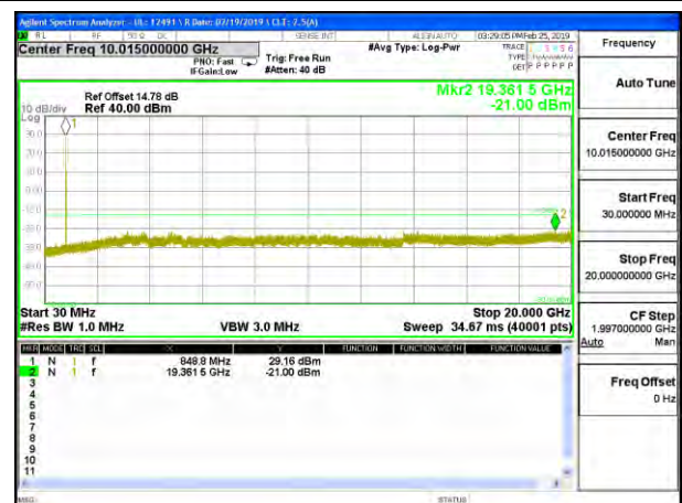
GSM 850MHz EGPRS High Channel
