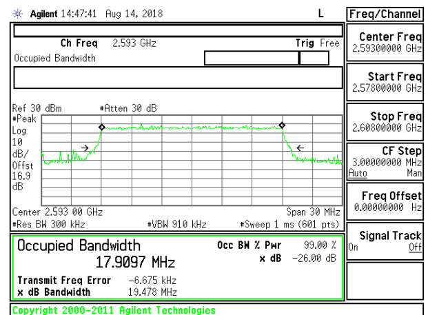
LTE B41 20MHz QPSK Middle Channel RB100-0 ID:12491
