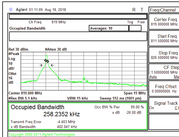
LTE B26 10MHz QPSK Middle Channel RB1-0, ID: 10646
