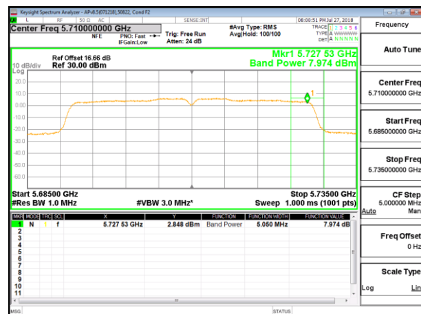
CHANNEL 142 POWER ANTENNA 4
