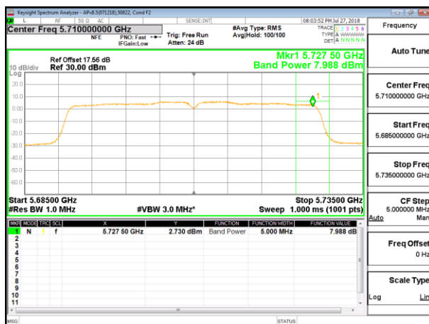
CHANNEL 142 POWER ANTENNA 5
