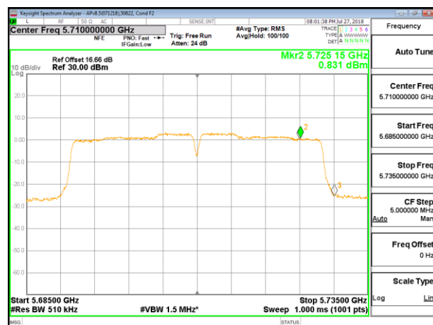
CHANNEL 142 PSD ANTENNA 4
