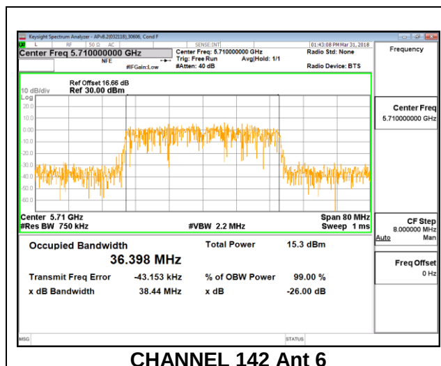
CHANNEL 142 Ant 6
