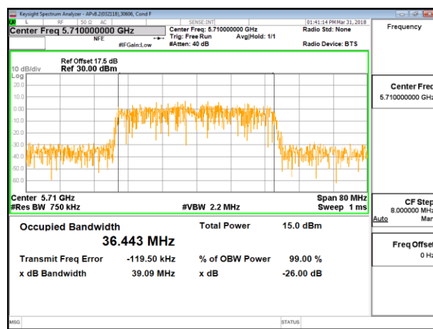
CHANNEL 142 Ant 5
