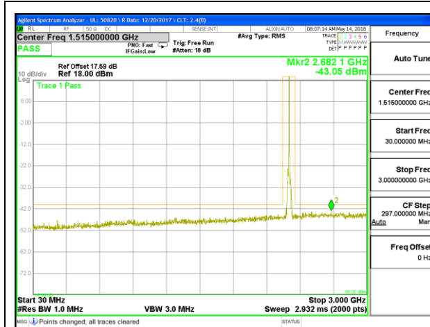
LTE B30 5MHz QPSK Low Channel RB1-0 30MHz-3GHz
