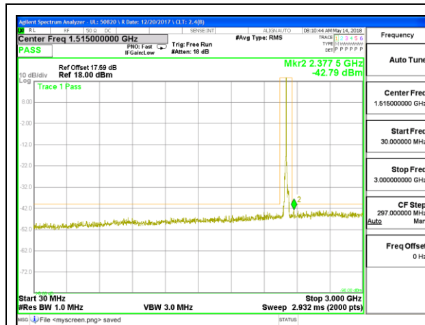
LTE B30 5MHz 16QAM Low Channel RB1-0 30MHz-3GHz
