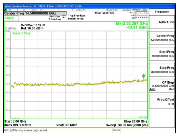
LTE B30 5MHz QPSK High Channel RB1-0 3GHz-26GHz
