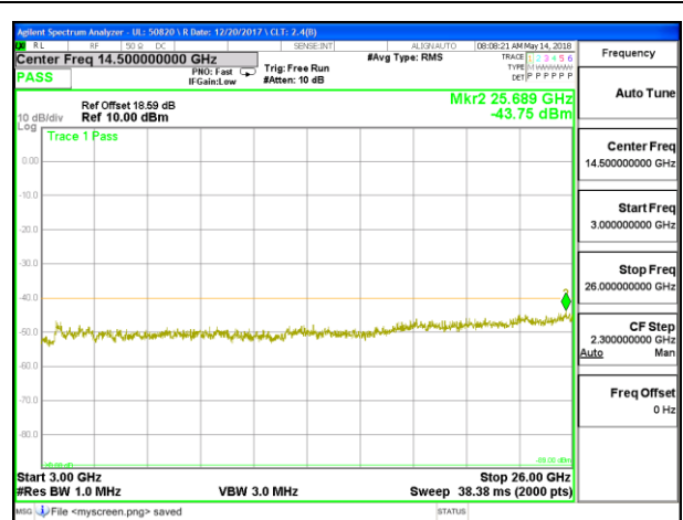
LTE B30 5MHz QPSK Low Channel RB1-0 3GHz-26GHz
