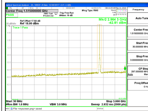
LTE B30 5MHz QPSK Middle Channel RB1-0 30MHz-3GHz
