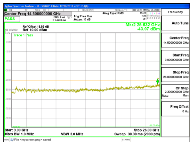
LTE B30 5MHz 16QAM Middle Channel RB1-0 3GHz-26GHz
