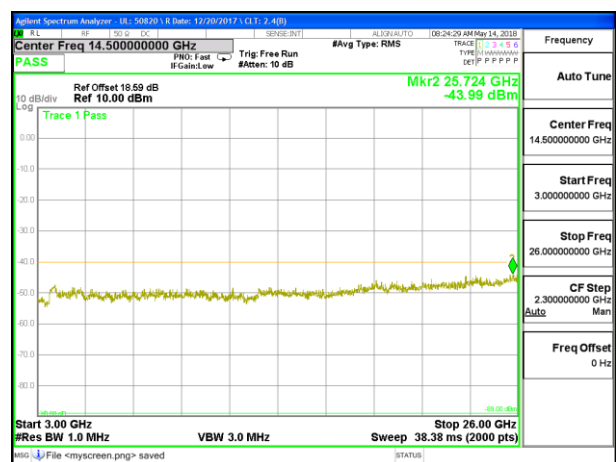
LTE B30 5MHz 16QAM High Channel RB1-0 3GHz-26GHz
