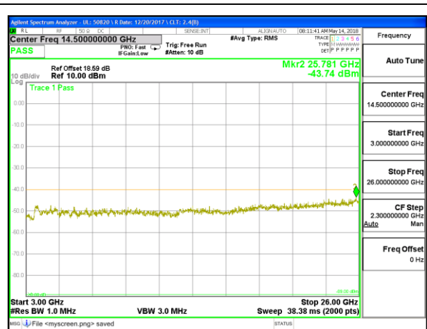
LTE B30 5MHz 16QAM Low Channel RB1-0 3GHz-26GHz
