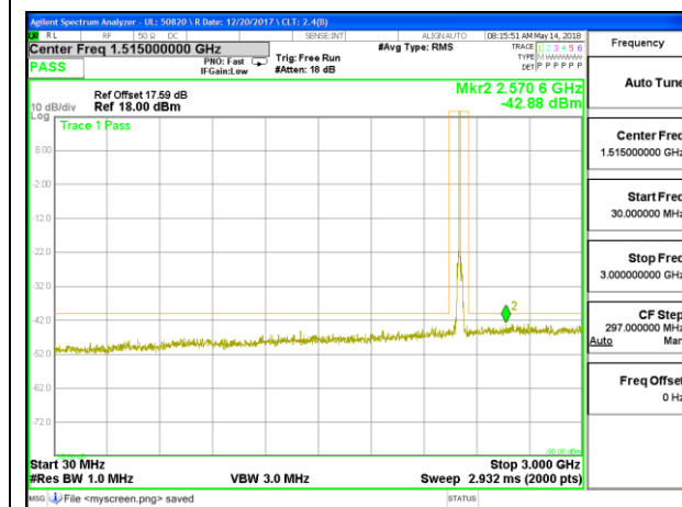
LTE B30 5MHz 16QAM Middle Channel RB1-0 30MHz-3GHz
