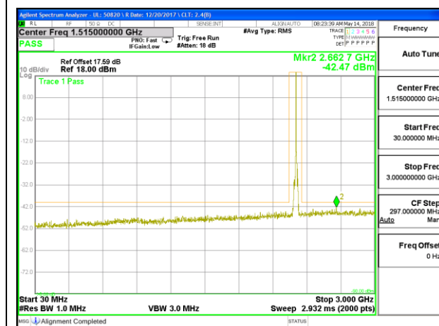
LTE B30 5MHz 16QAM High Channel RB1-0 30MHz-3GHz
