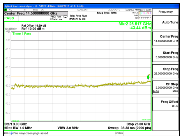
LTE B30 5MHz QPSK Middle Channel RB1-0 3GHz-26GHz
