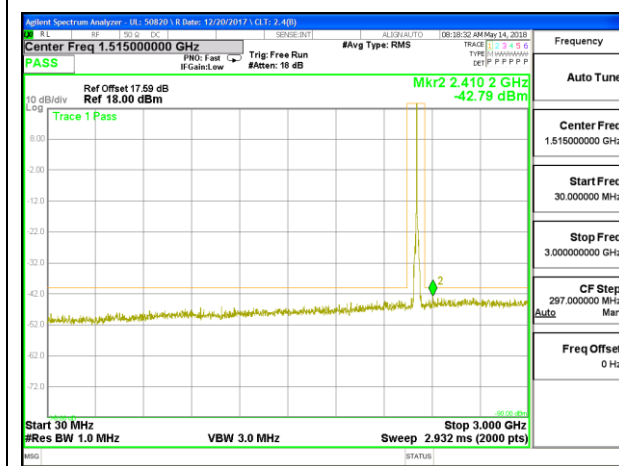
LTE B30 5MHz QPSK High Channel RB1-0 30MHz-3GHz
