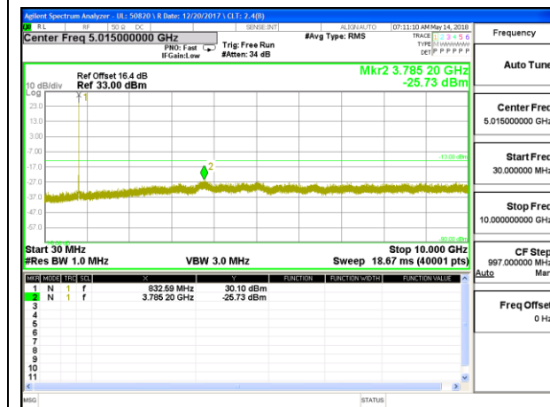
LTE B5 10MHz QPSK Middle Channel RB1-0
