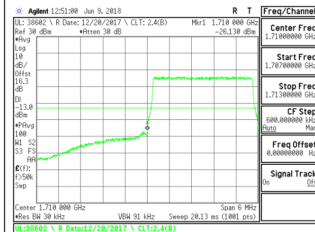
LTE B66 3MHz 16QAM Low Channel RB15-0
