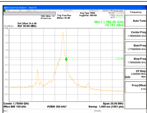
LTE B66 10MHz QPSK High Channel RB1-49 39004
