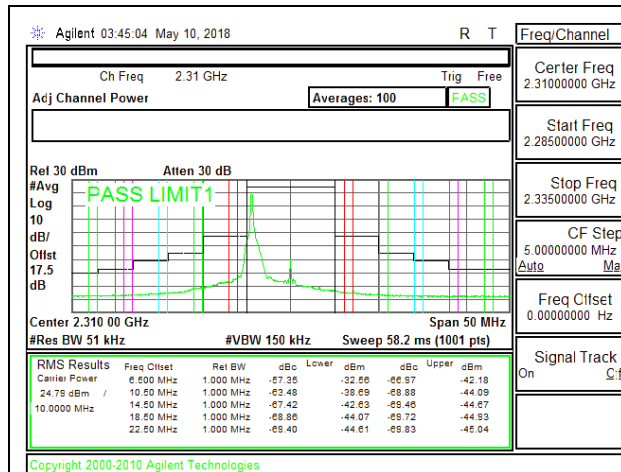
LTE B30 10MHz QPSK Middle Channel RB1-0 39004
