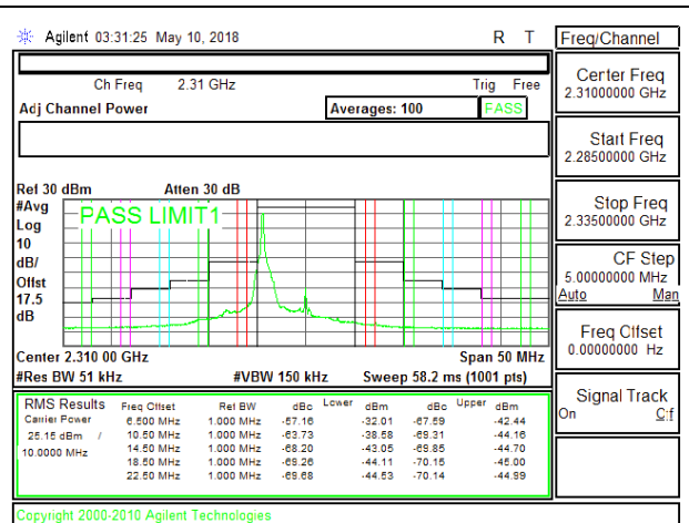
LTE B30 10MHz 16QAM Middle Channel RB1-0 39004
