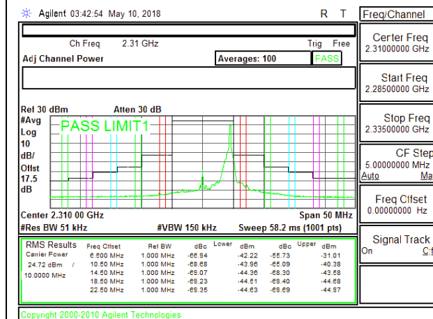
LTE B30 10MHz QPSK Middle Channel RB1-49 39004
