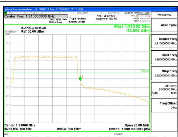
LTE B2 10MHz 16QAM High Channel RB50-0
