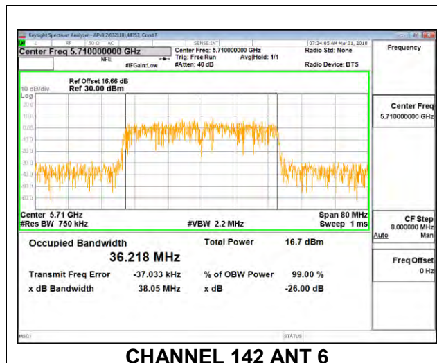
CHANNEL 142 ANT 6
