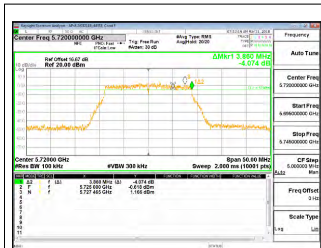
CHANNEL 144 ANT 6
