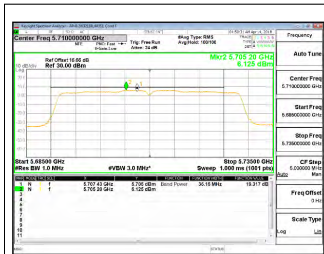
CHANNEL 142 ANT 6
