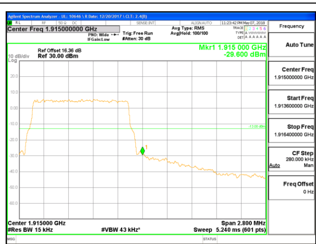
LTE B25 1.4MHz 16QAM High Channel RB6-0
