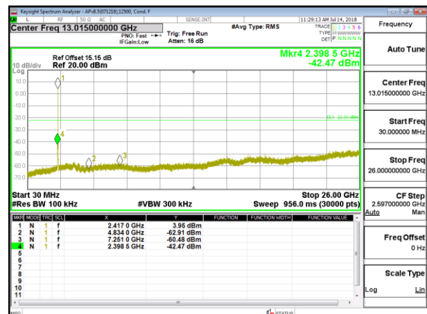
OUT-OF-BAND LOW CHANNEL 2 ANTENNA 3
