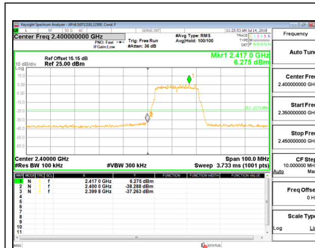
LOW CHANNEL 1 BANDEDGE ANTENNA 3
