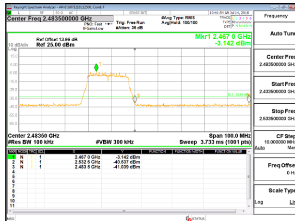
HIGH CHANNEL 13 BANDEDGE ANTENNA 4
