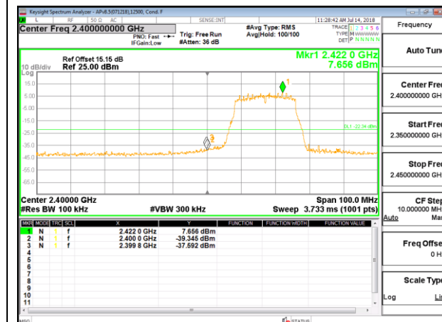
LOW CHANNEL 2 BANDEDGE ANTENNA 3
