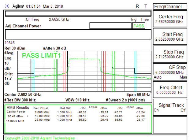
LTE B41 15MHz 16QAM High Channel RB75-0
