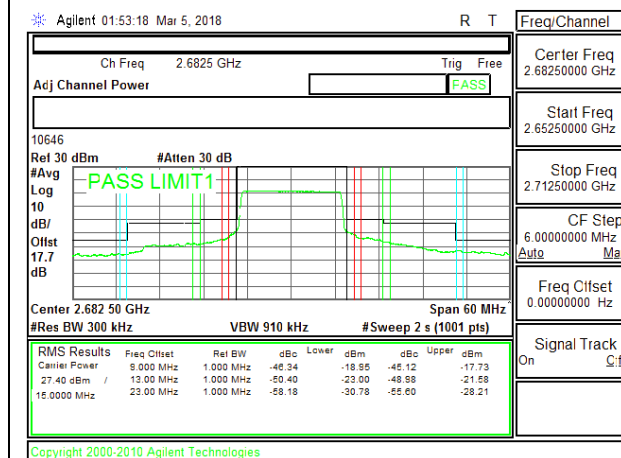
LTE B41 15MHz QPSK High Channel RB75-0
