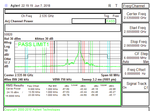
LTE B7 15MHz 16QAM Middle Channel RB1-74
