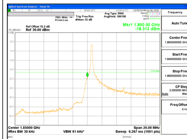
LTE B25 10MHz 16QAM Low Channel RB1-0 ID: 10646
