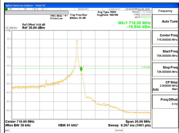
LTE B17 10MHz QPSK High Channel RB1-49 ID: 50820
