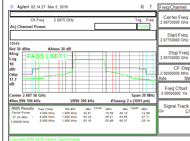
LTE B41 5MHz QPSK High Channel RB25-0
