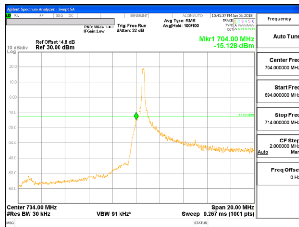
LTE B17 10MHz QPSK Low Channel RB1-0 ID: 50820
