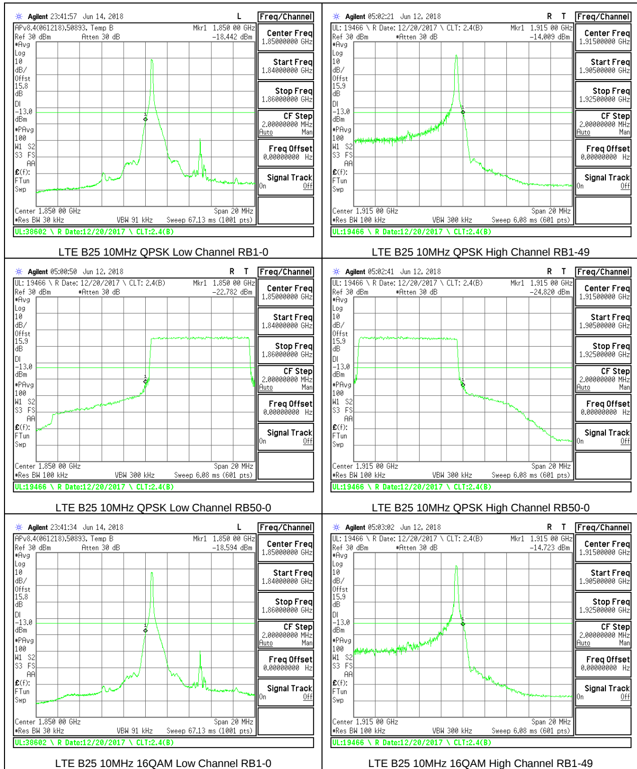
LTE B25 10MHz 16QAM Low Channel RB1-0
