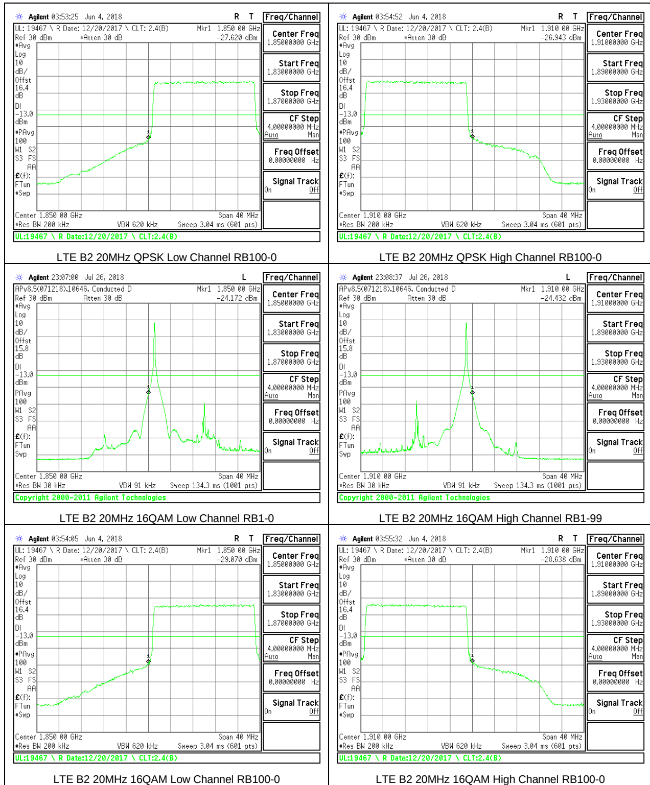
LTE B2 20MHz 16QAM Low Channel RB100-0
