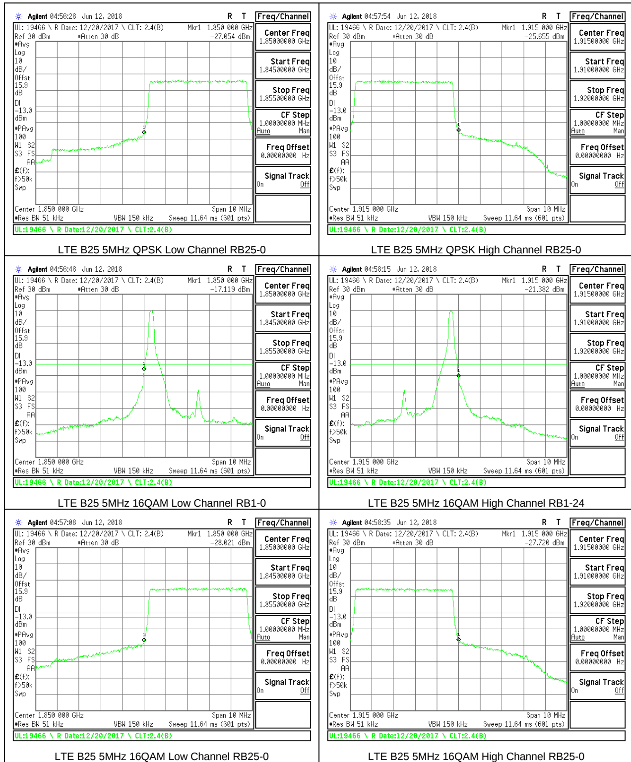
LTE B25 5MHz 16QAM Low Channel RB25-0
