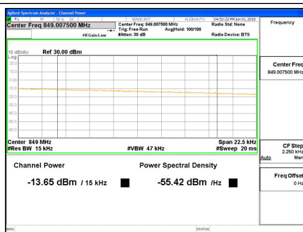
CDMA BC0 1xEV-DO Rev A High Channel ID:19424
