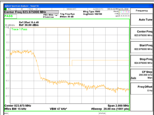
CDMA BC10 1xRTT High Channel, RBW=1% of EBW ID:19424
