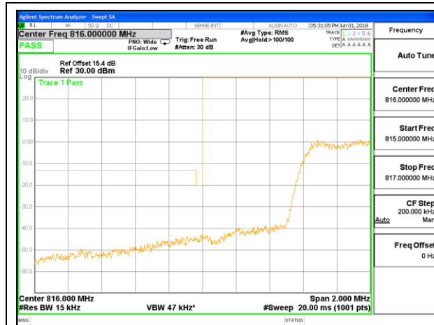
CDMA BC10 1xRTT Low Channel, RBW=1% of EBW ID:19424
