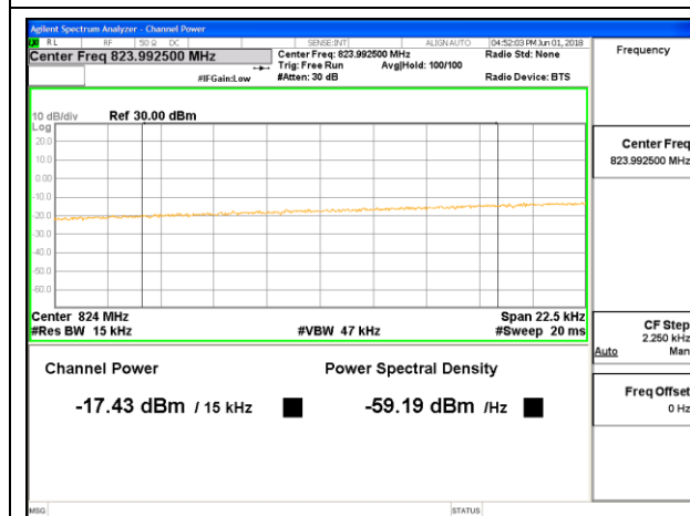
CDMA BC0 1xEV-DO Rev A Low Channel ID:19424
