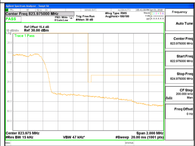
CDMA BC10 1xEV-DO Rev A High Channel, RBW=1% of EBW ID:19424
