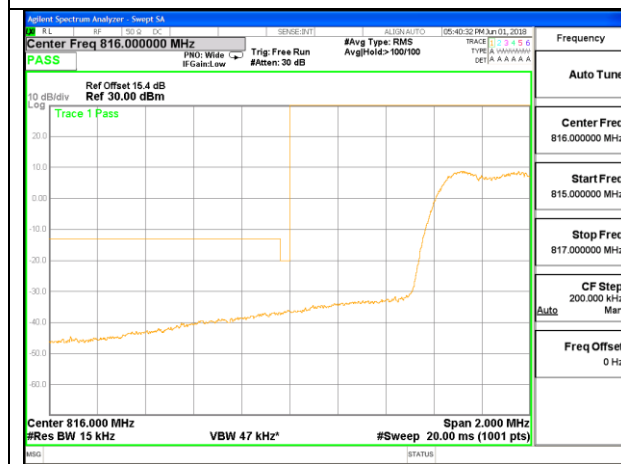
CDMA BC10 1xEV-DO Rev A Low Channel, RBW=1% of EBW ID:19424
