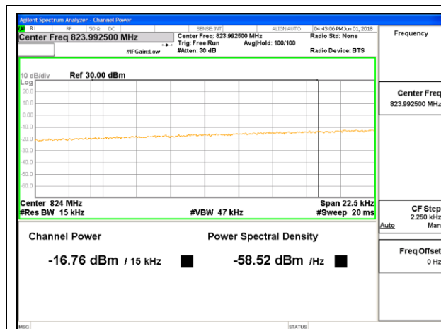
CDMA BC0 1xRTT Low Channel ID:19424
