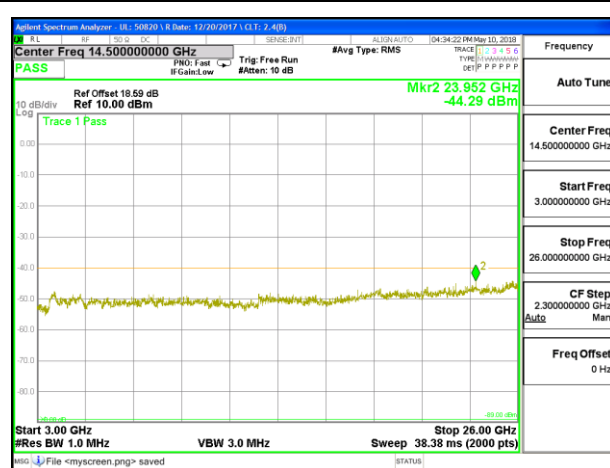
LTE B30 10MHz 16QAM High Channel RB1-0
