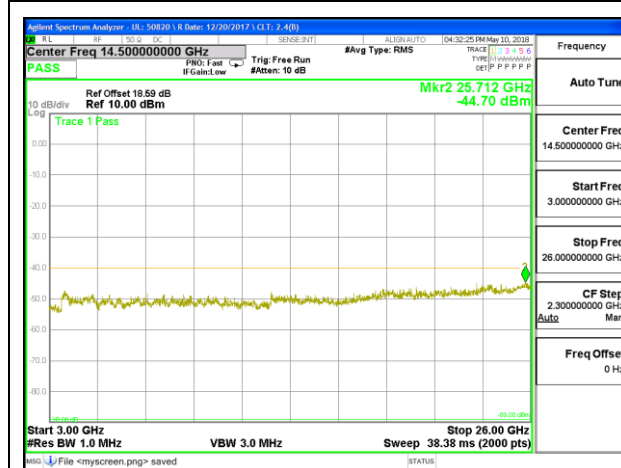
LTE B30 10MHz QPSK High Channel RB1-0
