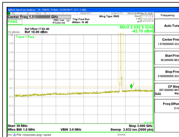
LTE B30 10MHz QPSK Mid Channel RB1-0
