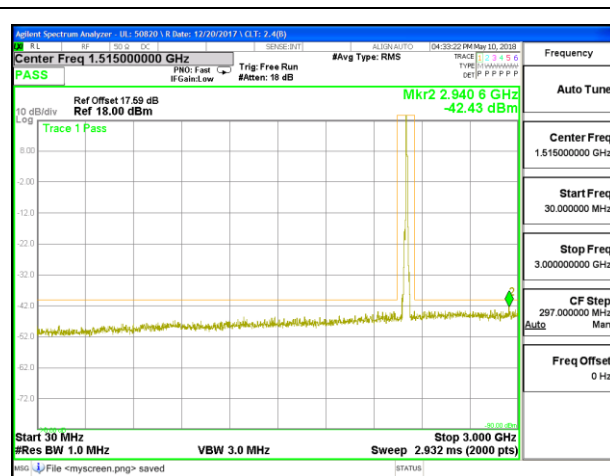
LTE B30 10MHz 16QAM Mid Channel RB1-0
