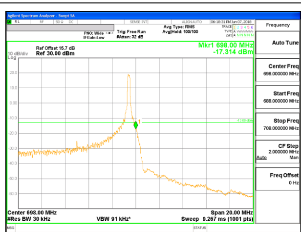
LTE B71 10MHz 16QAM High Channel RB1-49 ID19424
