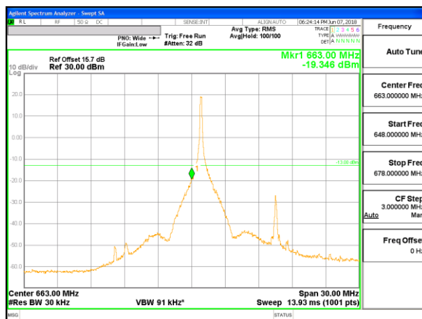
LTE B71 15MHz QPSK Low Channel RB1-0 ID19424
