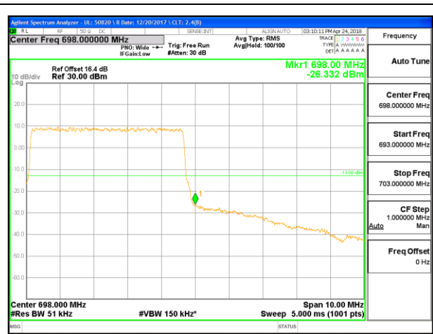
LTE B71 5MHz 16QAM High Channel RB25-0
