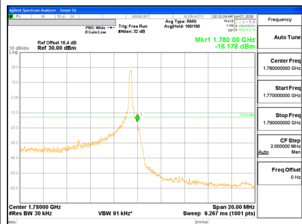
LTE B66 10MHz 16QAM High Channel RB1-49 ID19424
