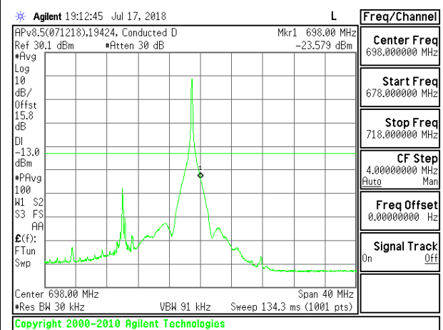
LTE B71 20MHz 16QAM High Channel RB1-99
