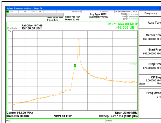
LTE B71 10MHz 16QAM Low Channel RB1-0 ID19424
