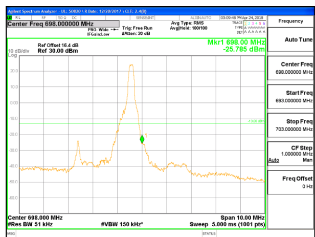
LTE B71 5MHz 16QAM High Channel RB1-24
