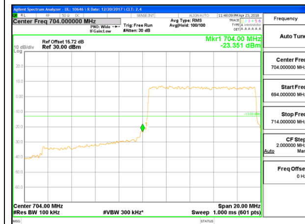
LTE B17 10MHz QPSK Low Channel RB50-0
