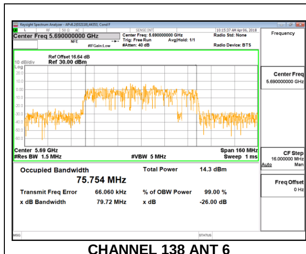
CHANNEL 138 ANT 6
