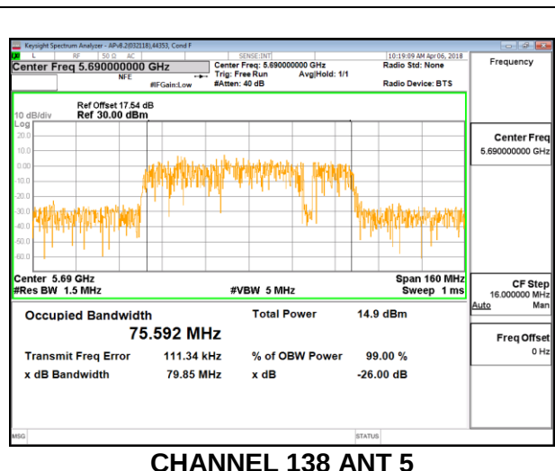
CHANNEL 138 ANT 5
