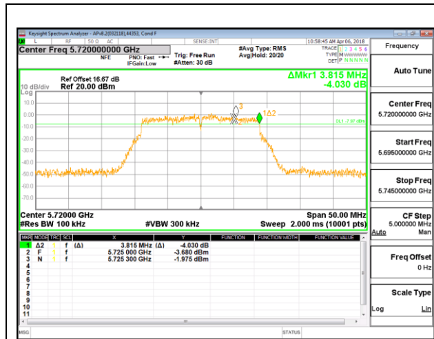
CHANNEL 144 ANT 6
