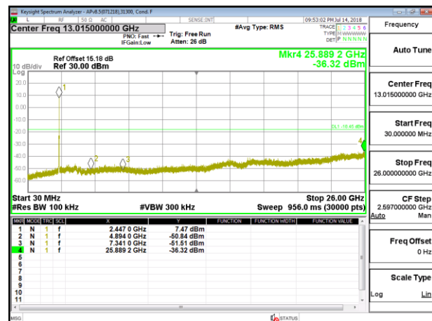
OUT-OF-BAND HIGH CHANNEL 8 ANTENNA 3
