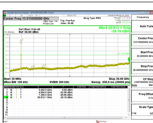
OUT-OF-BAND HIGH CHANNEL 9 ANTENNA 4
