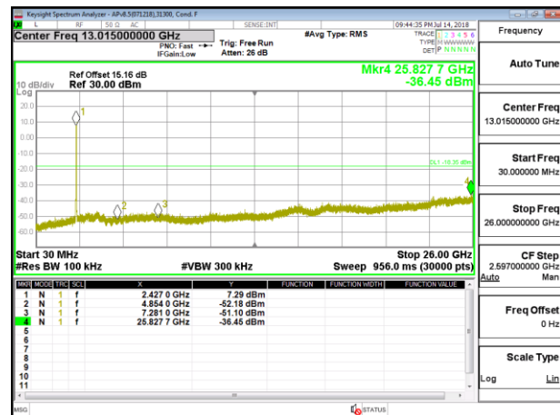
OUT-OF-BAND LOW CHANNEL 4 ANTENNA 3
