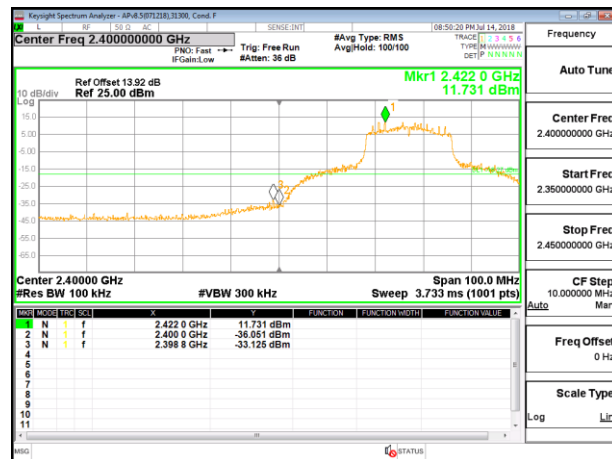
LOW CHANNEL 4 BANDEDGE ANTENNA 4
