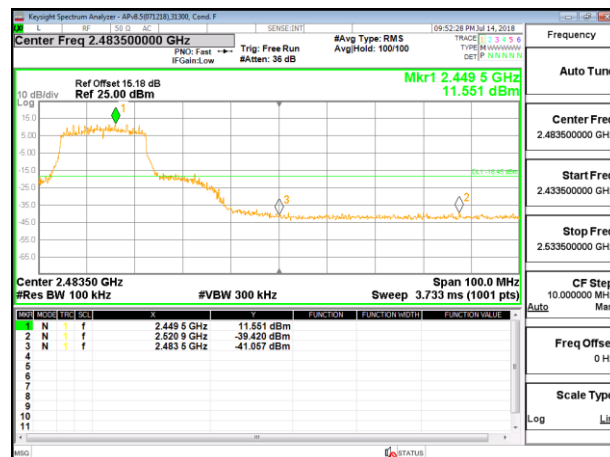
HIGH CHANNEL 8 BANDEDGE ANTENNA 3
