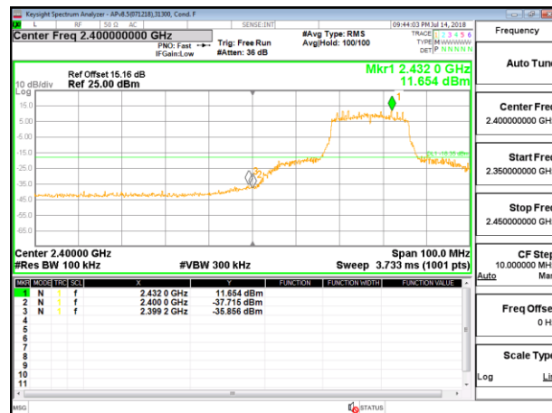
LOW CHANNEL 4 BANDEDGE ANTENNA 3
