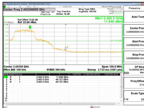
HIGH CHANNEL 8 BANDEDGE CHA ANTENNA 4
