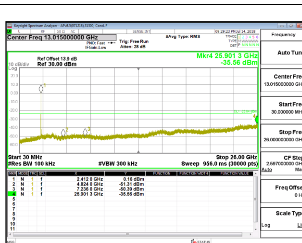
OUT-OF-BAND LOW CHANNEL 1 ANTENNA 4
