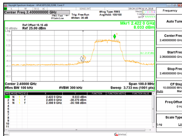
LOW CHANNEL 2 BANDEDGE ANTENNA 3
