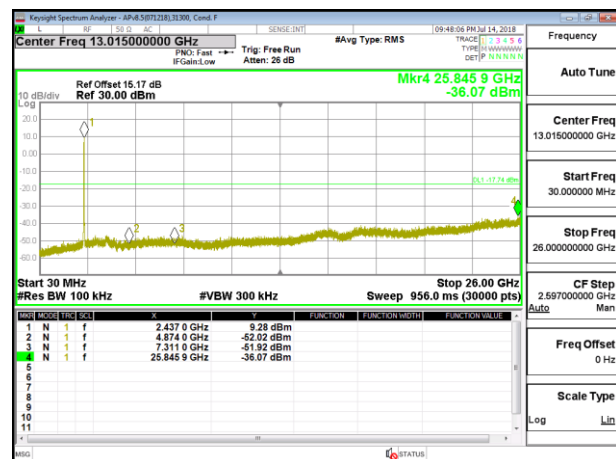
OUT-OF-BAND MID CHANNEL ANTENNA 3
