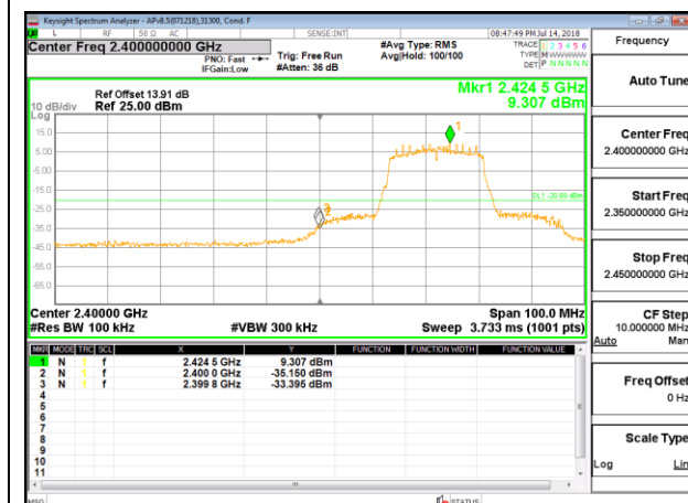
LOW CHANNEL 3 BANDEDGE ANTENNA 4
