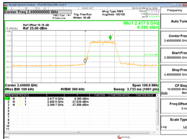
LOW CHANNEL 1 BANDEDGE ANTENNA 3
