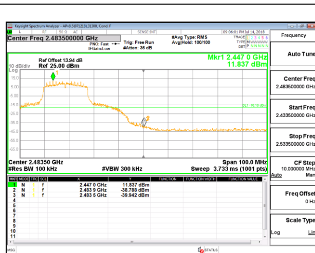
HIGH CHANNEL 9 BANDEDGE CHA ANTENNA 4
