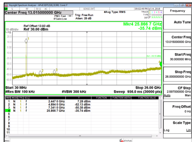
OUT-OF-BAND HIGH CHANNEL 8 ANTENNA 4
