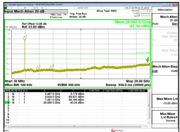
OUT-OF-BAND HIGH CHANNEL 12 ANTENNA 4
