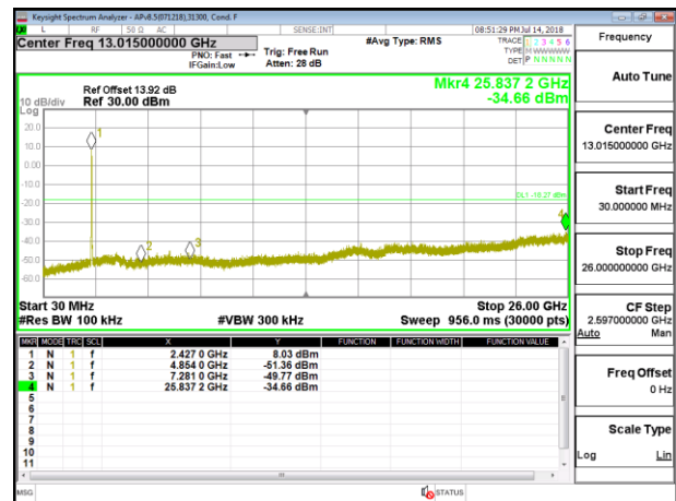
OUT-OF-BAND LOW CHANNEL 4 ANTENNA 4
