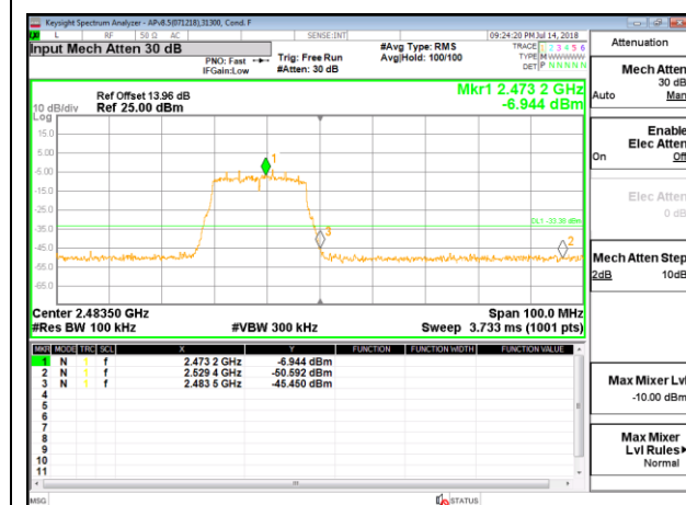
HIGH CHANNEL 13 BANDEDGE ANTENNA 4
