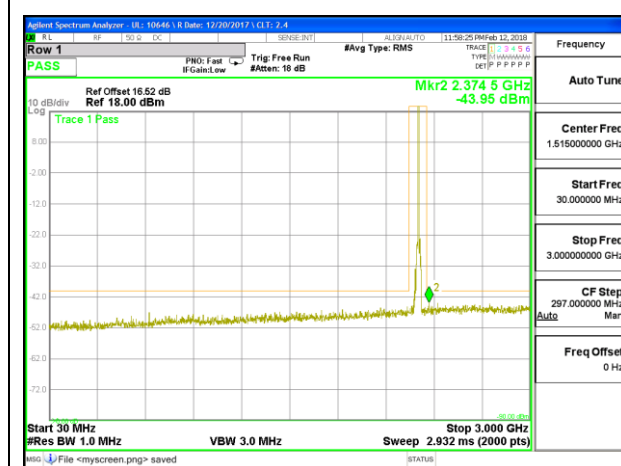
LTE B30 5MHz QPSK Mid Channel RB1-0
