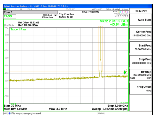
LTE B30 5MHz 16QAM Mid Channel RB1-0
