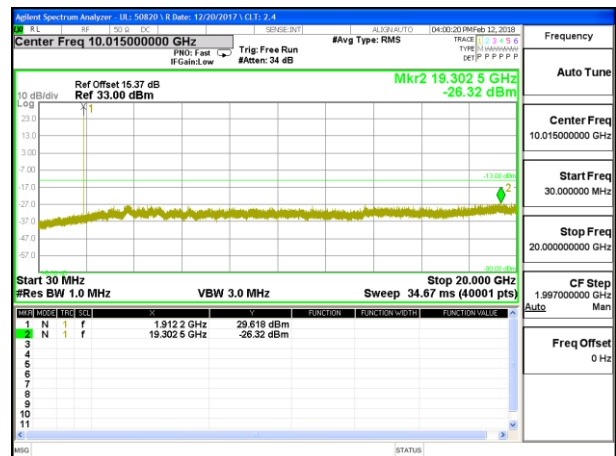
LTE B25 3MHz 16QAM High Channel RB1-0
