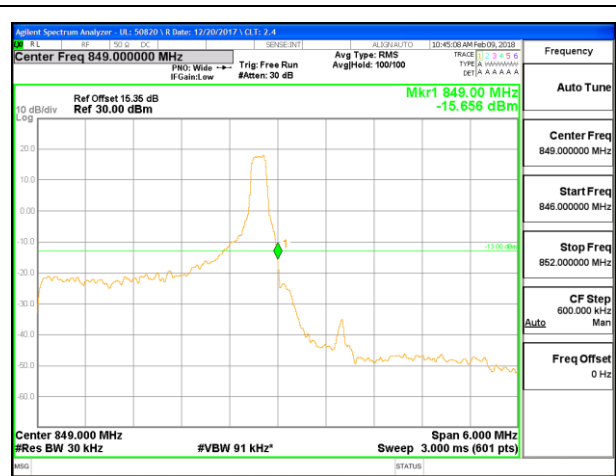
LTE B5 3MHz 16QAM High Channel RB1-14
