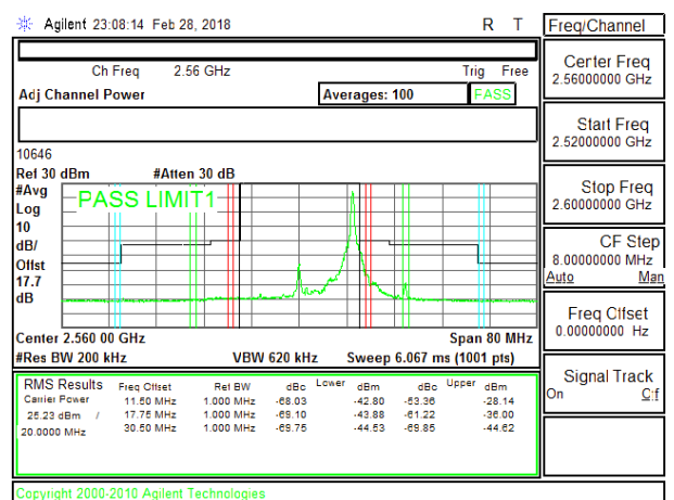
LTE B7 20MHz 16QAM High Channel RB1-99
