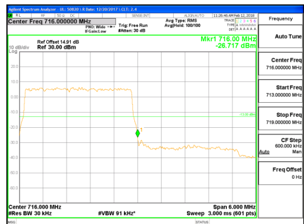
LTE B12 3MHz QPSK High Channel RB15-0
