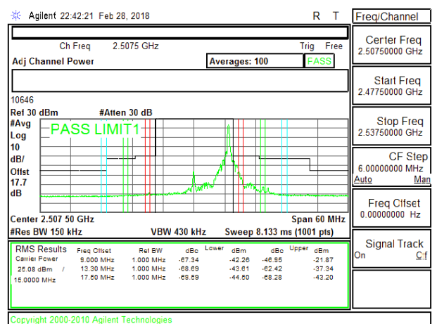
LTE B7 15MHz 16QAM Low Channel RB1-74
