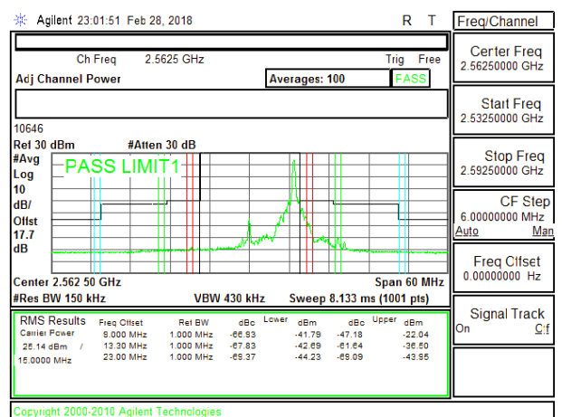
LTE B7 15MHz 16QAM High Channel RB1-74
