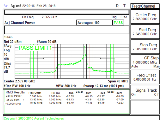
LTE B7 10MHz 16QAM High Channel RB1-49
