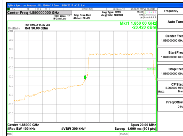
LTE B2 10MHz QPSK Low Channel RB50-0
