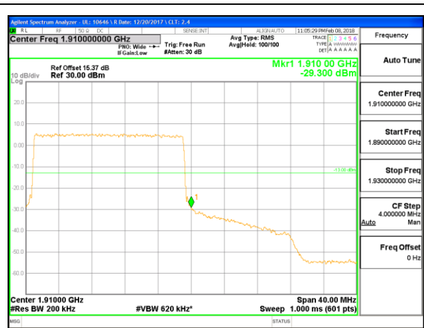
LTE B2 20MHz QPSK High Channel RB100-0
