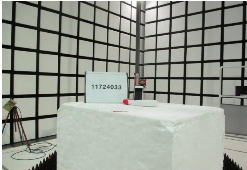
Z-AXIS PHOTO
