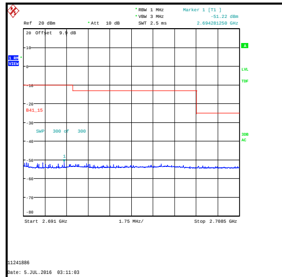
16QAM / 1 RB 0 Offset / 2691 to 2708.5 MHz **See note 8
