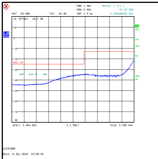
QPSK / 50 RB 0 Offset / 2484 to 2495 MHz
