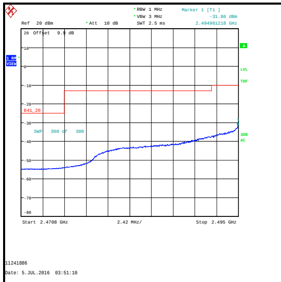
QPSK / 100 RB 0 Offset / 2470.8 to 2495 MHz
