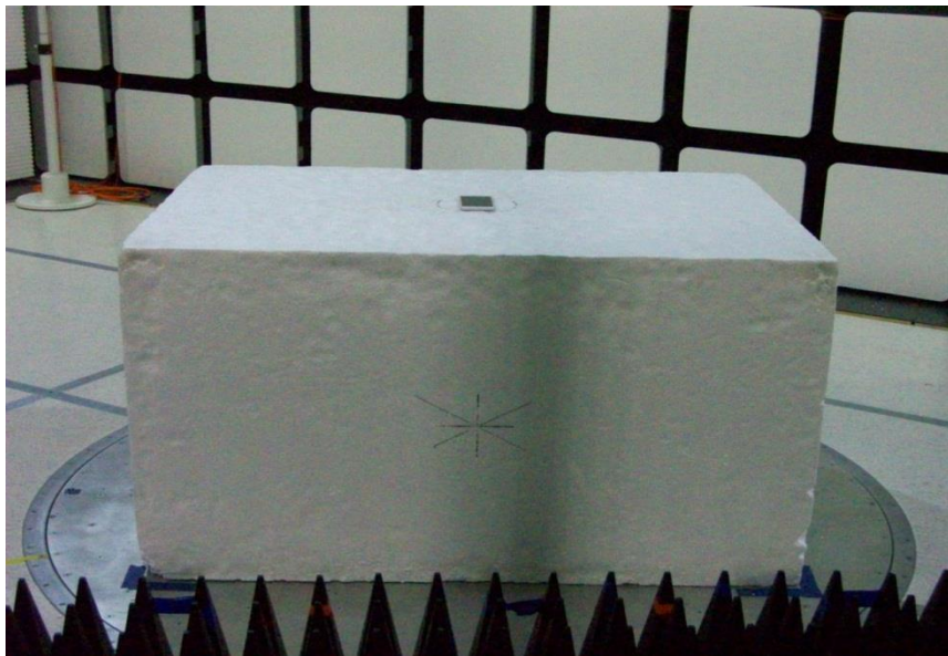
X-AXIS PHOTO
