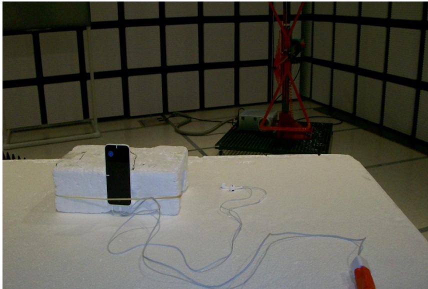
Z-AXIS PHOTO
