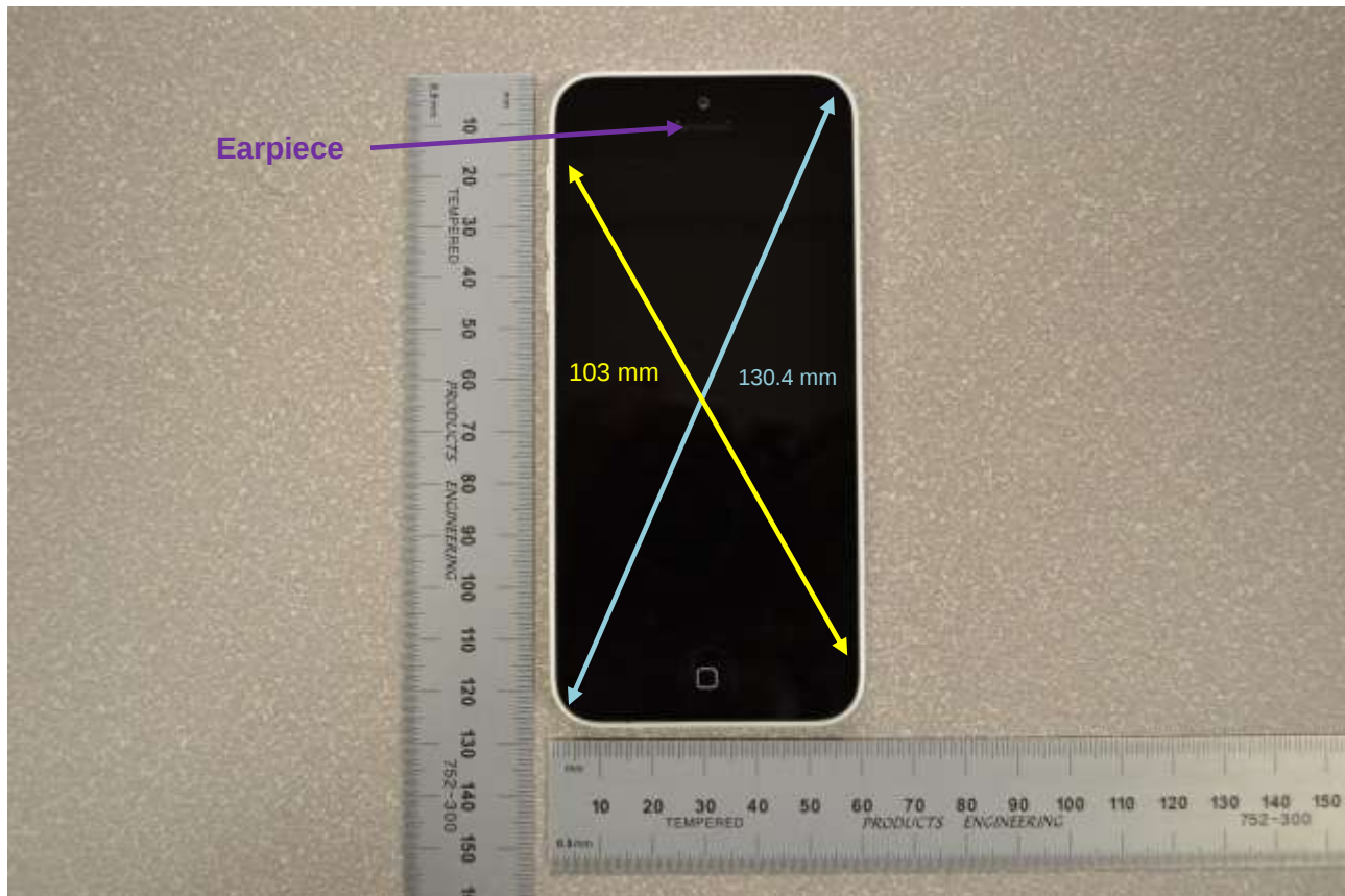
Overall Dimensions
