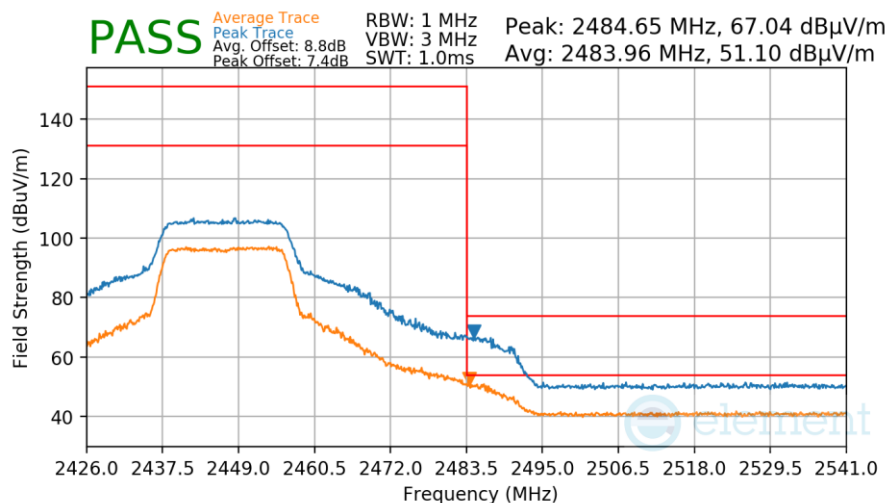
Plot 7-80. Radiated Restricted Upper Band Edge Measurement
