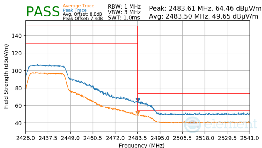
Plot 7-79. Radiated Restricted Upper Band Edge Measurement
