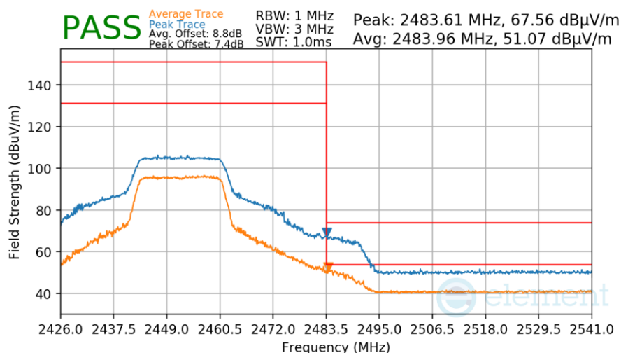
Plot 7-81. Radiated Restricted Upper Band Edge Measurement
