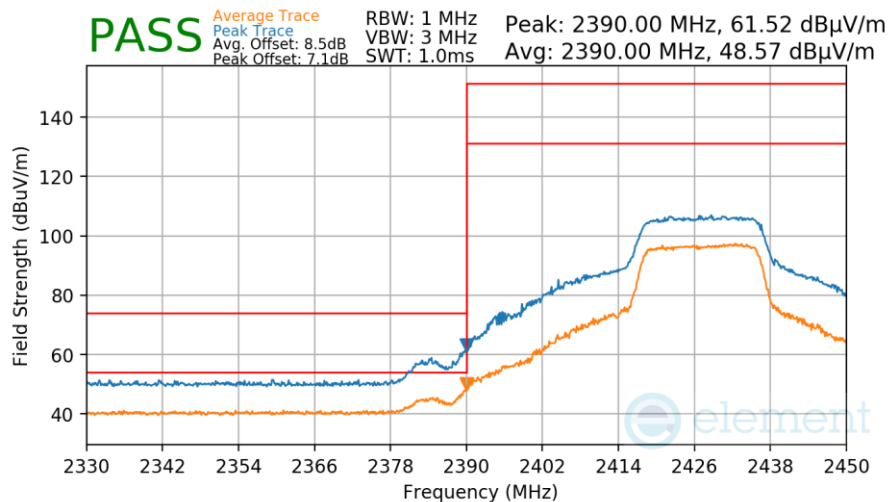
Plot 7-77. Radiated Restricted Lower Band Edge Measurement
