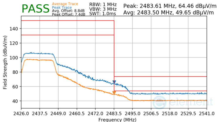
Plot 7-78. Radiated Restricted Upper Band Edge Measurement
