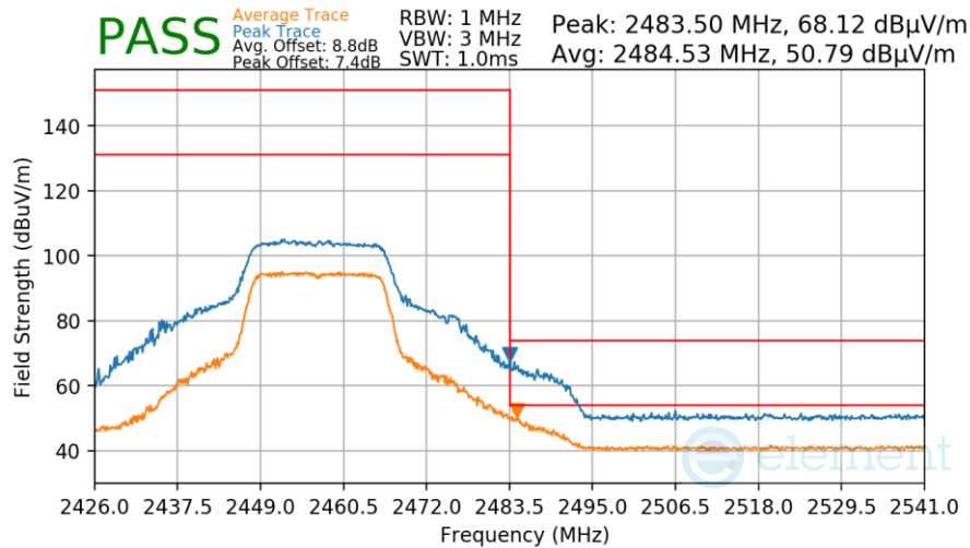
Plot 7-82. Radiated Restricted Upper Band Edge Measurement
