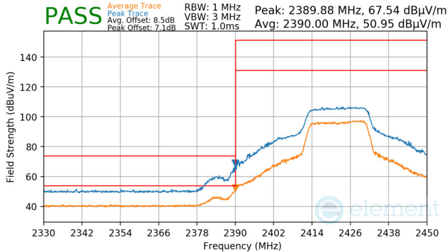
Plot 7-76. Radiated Restricted Lower Band Edge Measurement
