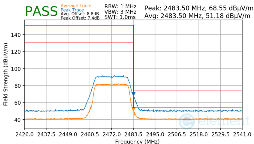
Plot 7-85. Radiated Restricted Upper Band Edge Measurement
