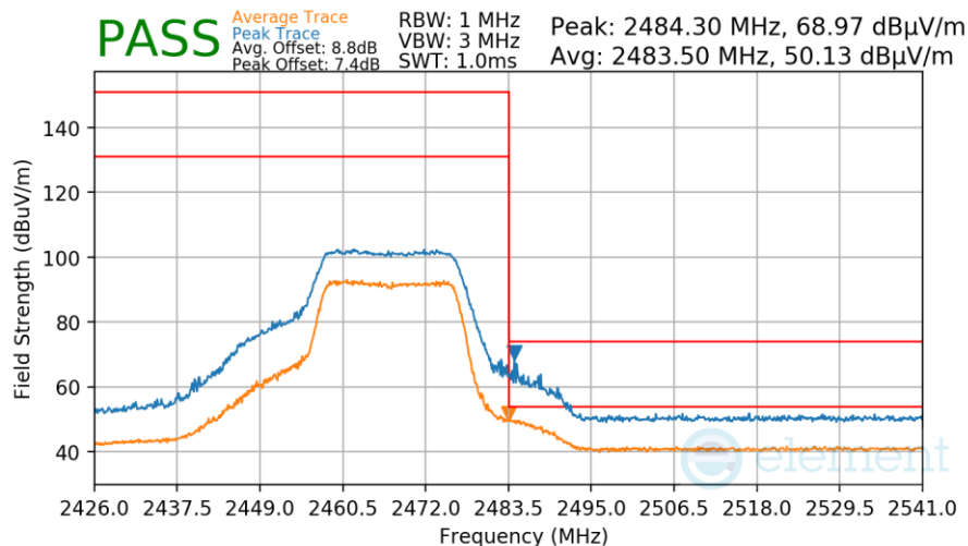
Plot 7-84. Radiated Restricted Upper Band Edge Measurement
