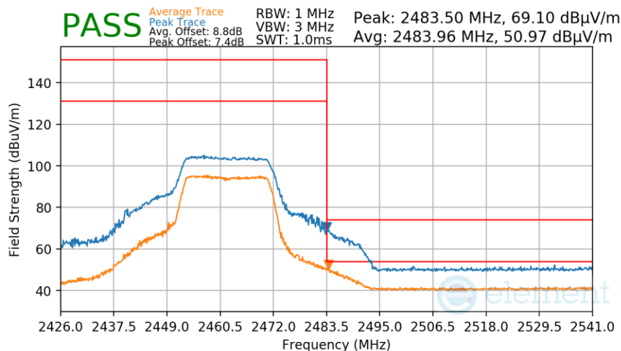
Plot 7-83. Radiated Restricted Upper Band Edge Measurement
