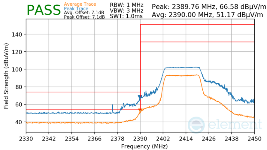
Plot 7-64. Radiated Restricted Lower Band Edge Measurement
