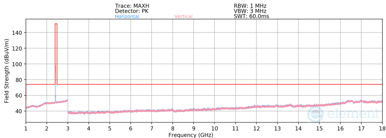
Plot 7-56. Radiated Spurious Emissions above 1GHz (802.11b – Ch. 1)
