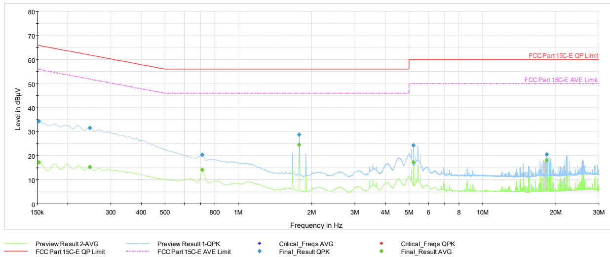
Plot 7-87. AC Line Conducted Plot 802.11b - Ch.6 (L1, with AC/DC adaptor via USB-C cable with magnetic charger)
