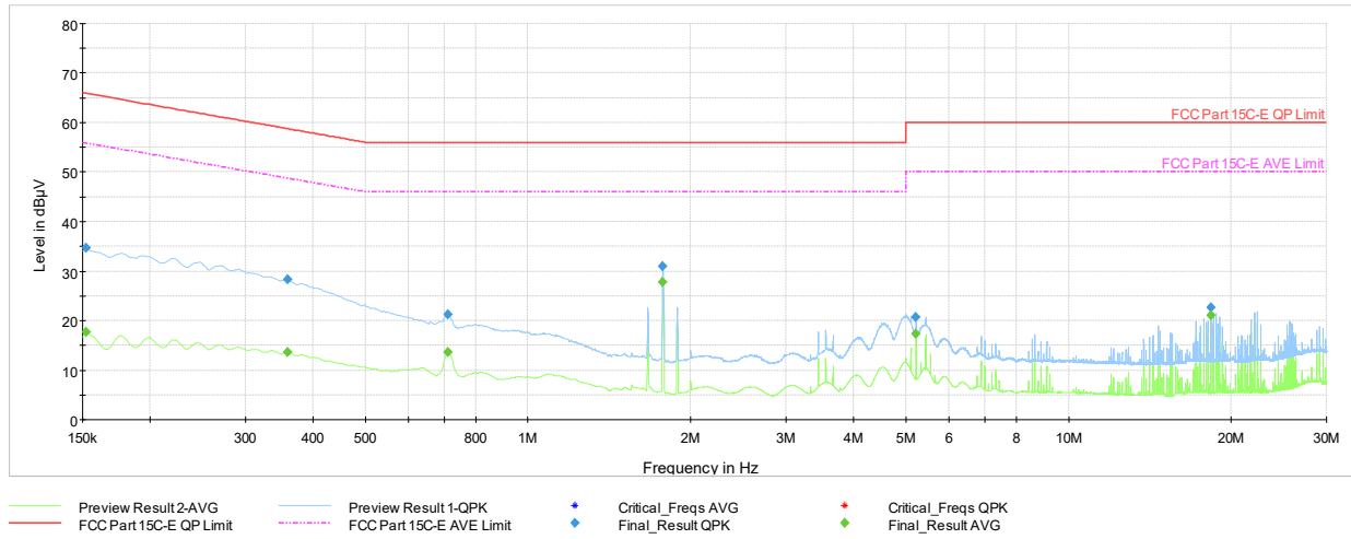
Plot 7-88. AC Line Conducted Plot 802.11b - Ch.6 (N, with AC/DC adaptor via USB-C cable with magnetic charger)
