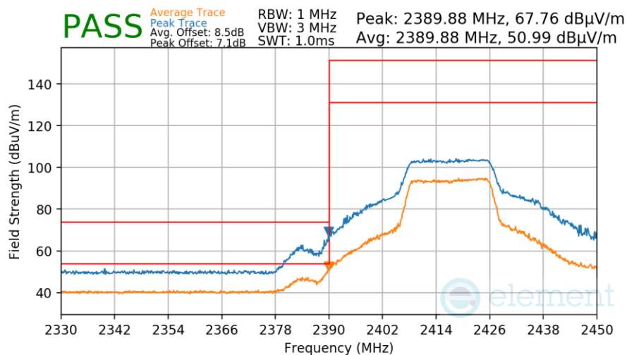
Plot 7-75. Radiated Restricted Lower Band Edge Measurement
