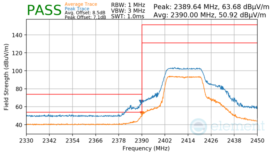
Plot 7-74. Radiated Restricted Lower Band Edge Measurement
