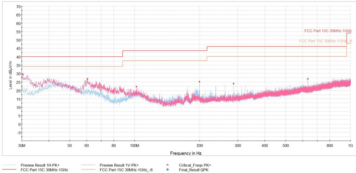
Plot 7-86. Radiated Spurious Emissions below 1GHz 11b Ch.6, with AC/DC Adapter via USB-C cable with magnetic charger
