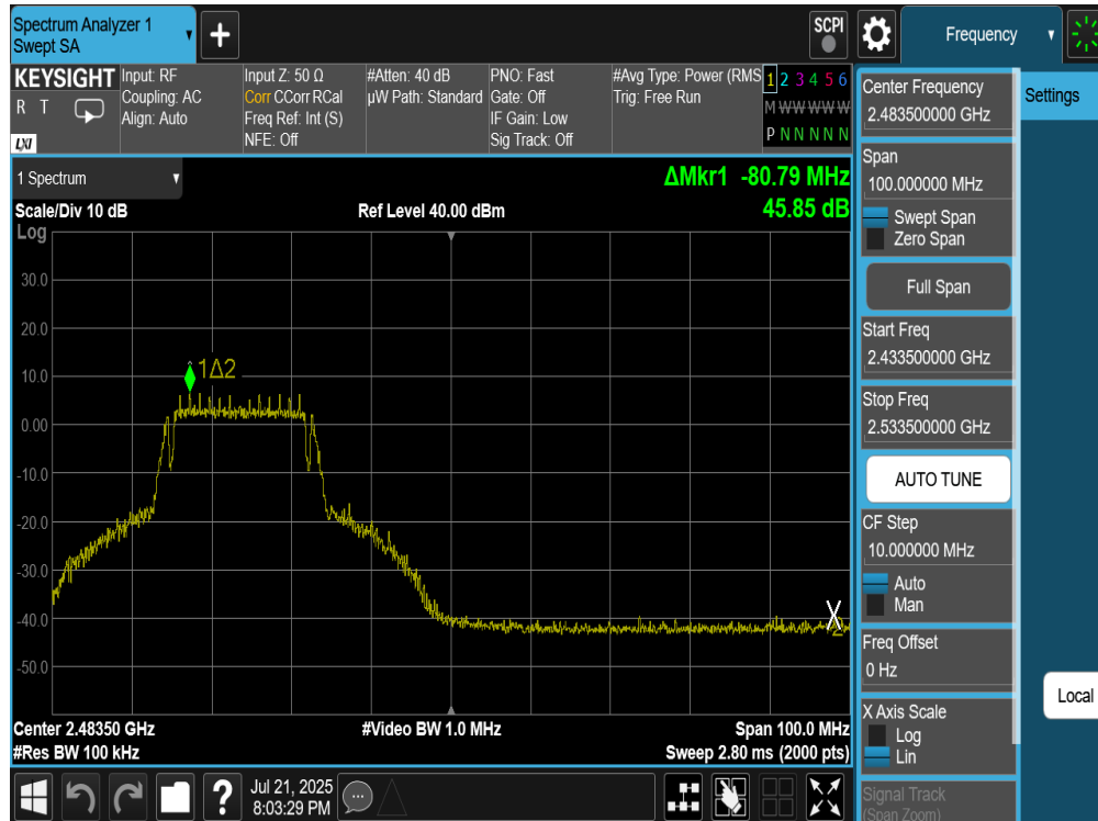
Plot 7-33. Band Edge Plot (802.11g – Ch. 10) – 6Mbps
