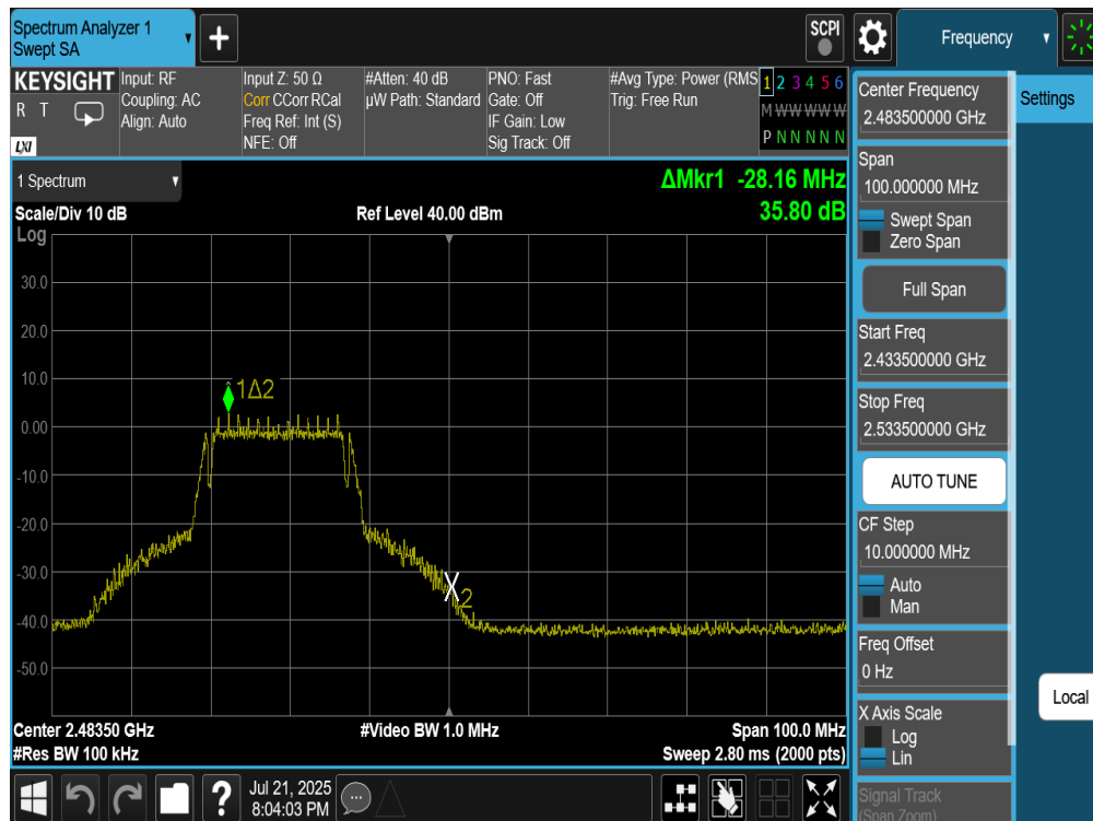
Plot 7-34. Band Edge Plot (802.11g – Ch. 11) – 6Mbps
