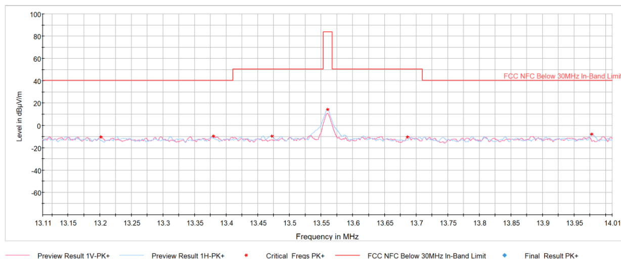
Plot 7-7. In Band Radiated Spurious Emissions (Reader A 848kbps, with AC/DC Adapter and Magnetic Charger)
