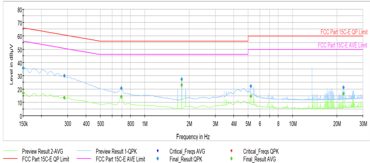
Plot 7-13. AC Line-Conducted Plot (N, CE F 212kbps, with AC/DC Adapter and Magnetic Charger)
