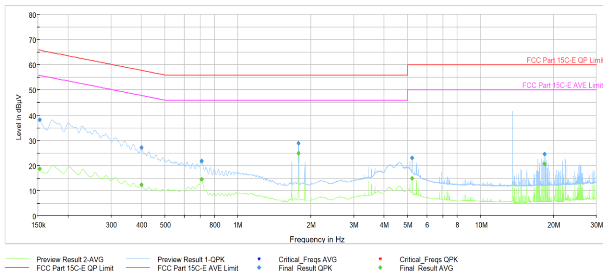
Plot 7-15. AC Line-Conducted Plot (N, Reader A 848kbps, with AC/DC Adapter and Magnetic Charger)
