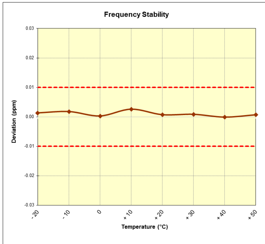
Figure 7-3. Frequency Stability Plot (CE F 212kbps)
