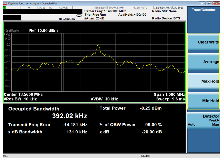
Plot 7-5. 20dB and 99% Bandwidth Plot (Reader 100% ASK 1 out of 256)
