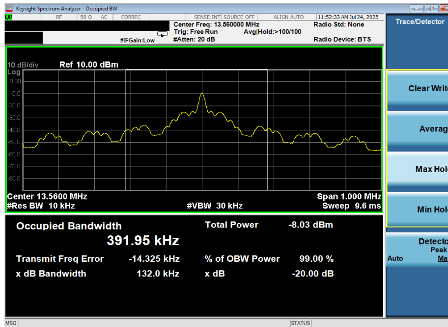
Plot 7-4. 20dB and 99% Bandwidth Plot (Reader 100% ASK 1 out of 4)
