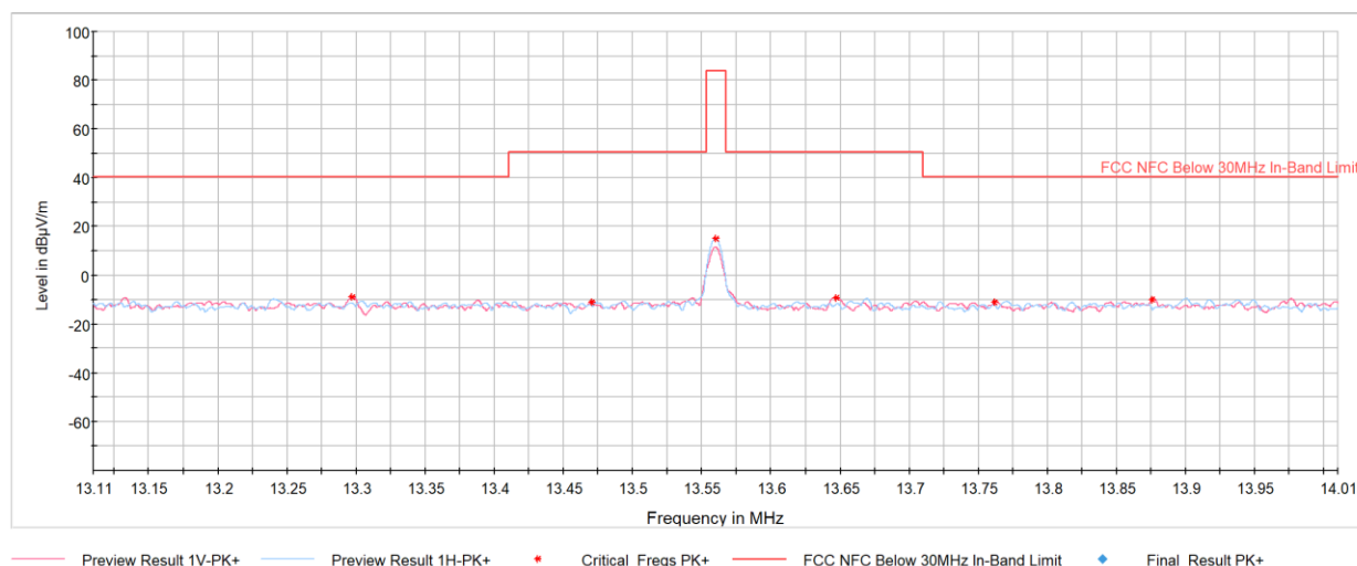
Plot 7-6. In Band Radiated Spurious Emissions (CE F 212kbps, with AC/DC Adapter and Magnetic Charger)
