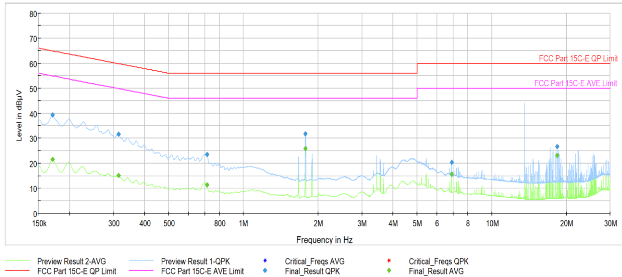
Plot 7-12. AC Line-Conducted Plot (L1, CE F 212kbps, with AC/DC Adapter and Magnetic Charger)
