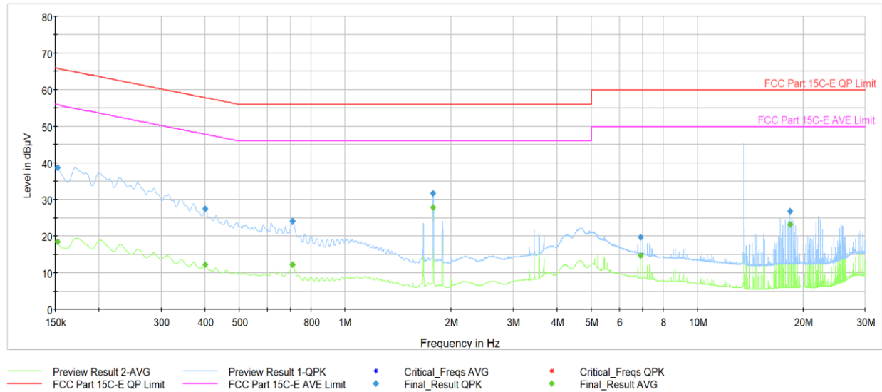
Plot 7-14. AC Line-Conducted Plot (L1, Reader A 848kbps, with AC/DC Adapter and Magnetic Charger)
