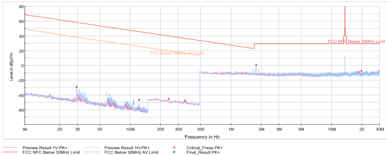
Plot 7-8. Radiated Spurious Emissions 9kHz – 30MHz (CE F 212kbps, with AC/DC Adapter and Magnetic Charger)
