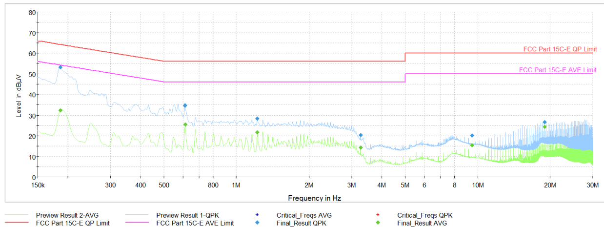
Plot 6-13. AC Line Conducted Plot (L1 - Mode 1, with Host Laptop via USB-C Cable)
