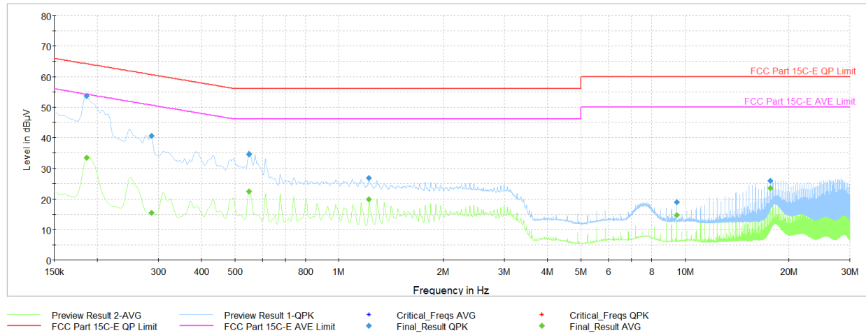
Plot 6-14. AC Line Conducted Plot (N - Mode 1, with Host Laptop via USB-C Cable)
