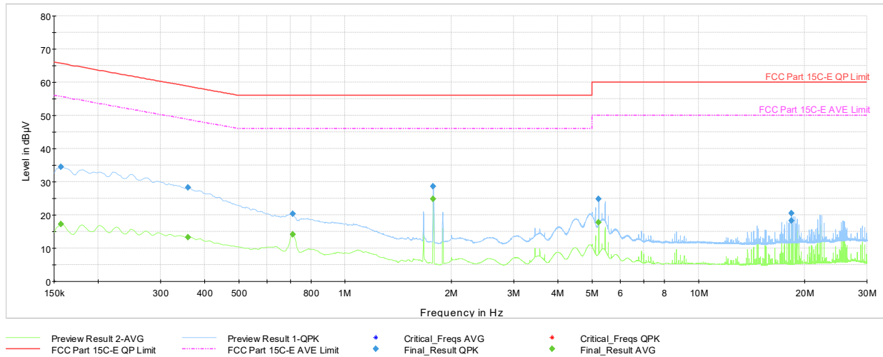
Plot 7-38. AC Line Conducted Plot with Bluetooth LE (L1, 1Mbps ePA – Ch.19 with AC/DC adaptor via USB-C cable with magnetic charger)
