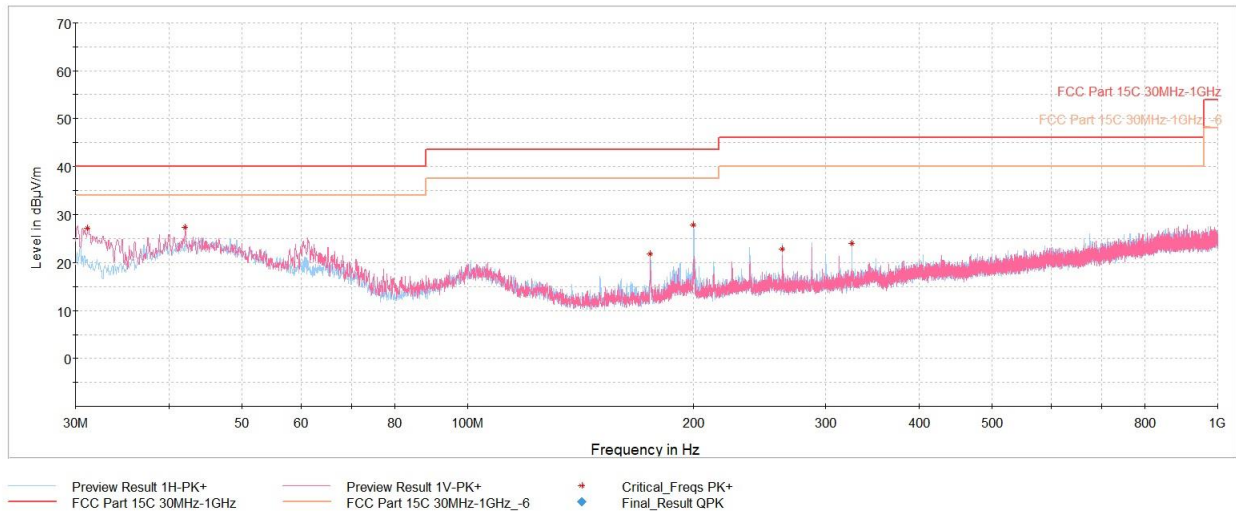
Plot 7-37. Radiated Spurious Emissions Below 1GHz (1Mbps, ePA – Ch.19, Pol. H & V, with AC/DC adaptor via USB-C cable with magnetic charger)
