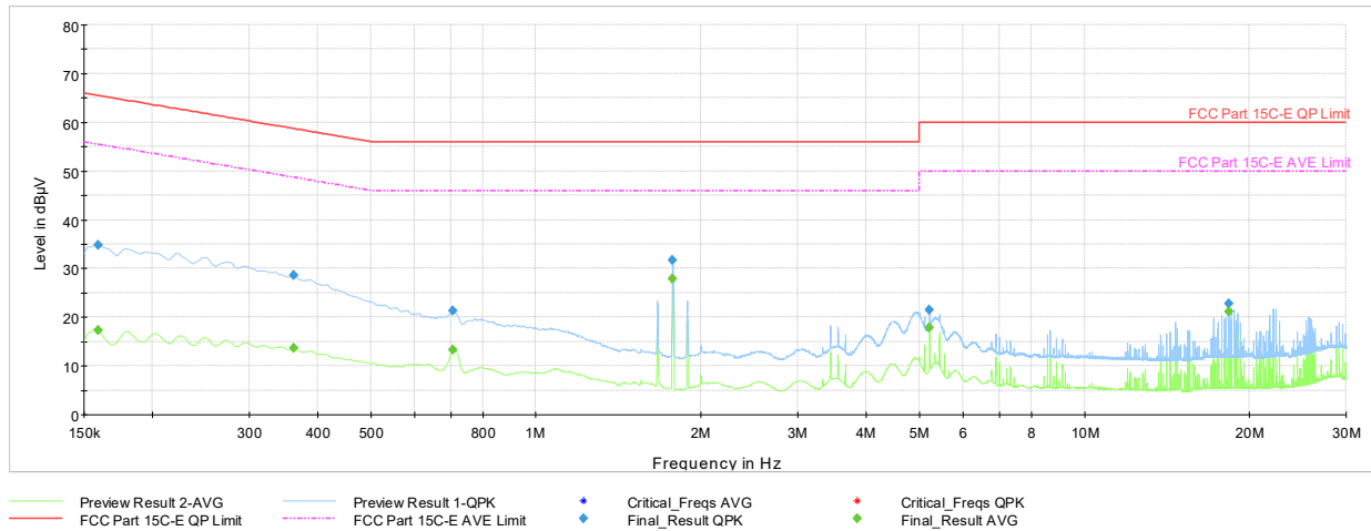
Plot 7-39. AC Line Conducted Plot with Bluetooth LE (N, 1Mbps ePA – Ch.19, with AC/DC adaptor via USB-C cable with magnetic charger)
