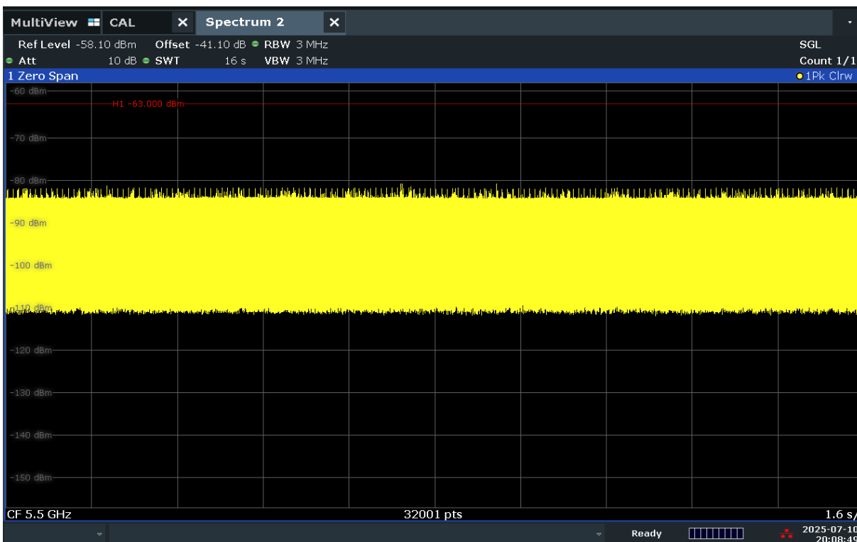
Figure 9-1. 5500MHz - Channel Loading - (20MHz)
