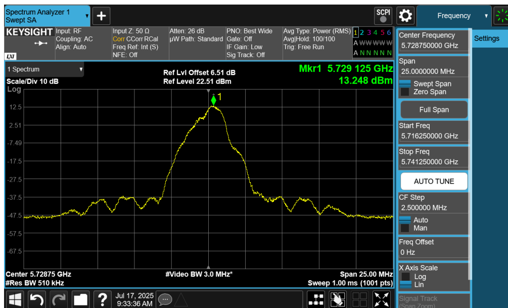
Plot 7-16. PSD (O-QPSK, 5728.75MHz, 1000kpbs)
