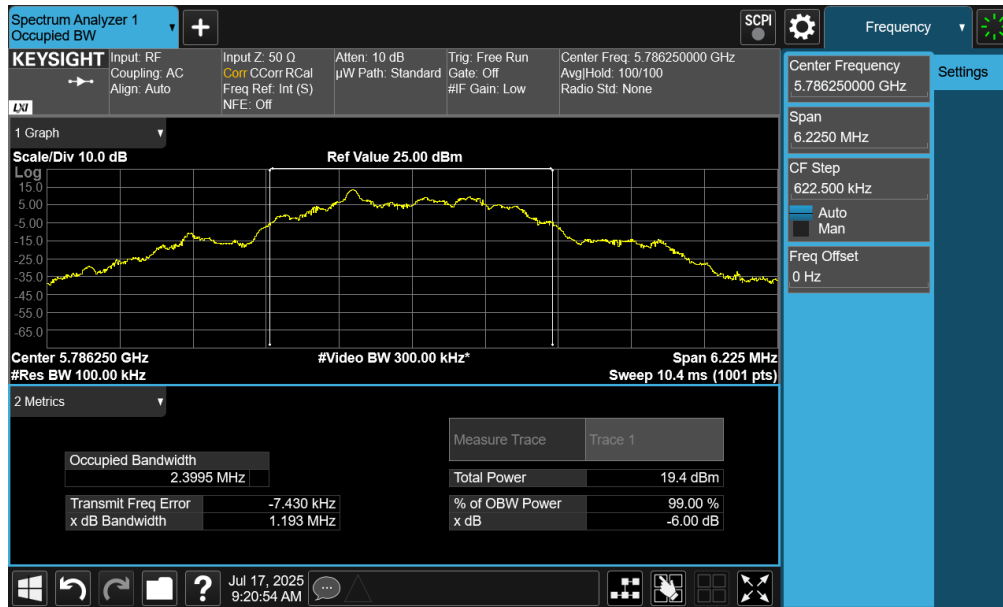
Plot 7-5. 6dB BW & 99% OBW (O-QPSK, 5786.25MHz, 500kpbs)
