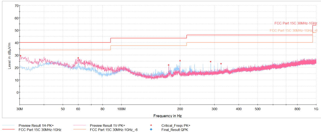
Plot 7-29. RSE 30MHz - 1GHz (O-QPSK, 250Kbps – Ch. 24), with AC/DC Adapter & magnetic charger
