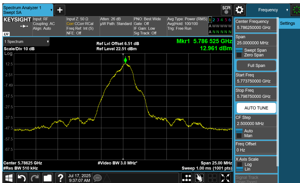
Plot 7-17. PSD (O-QPSK, 5786.25MHz, 1000kpbs)
