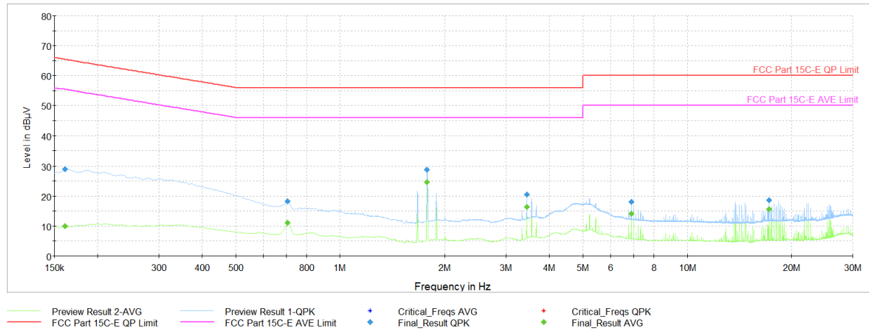
Plot 7-30. AC Line Conducted Plot (O-QPSK, 250Kbps – Ch. 24) (L1) with AC/DC Adapter & magnetic charger
