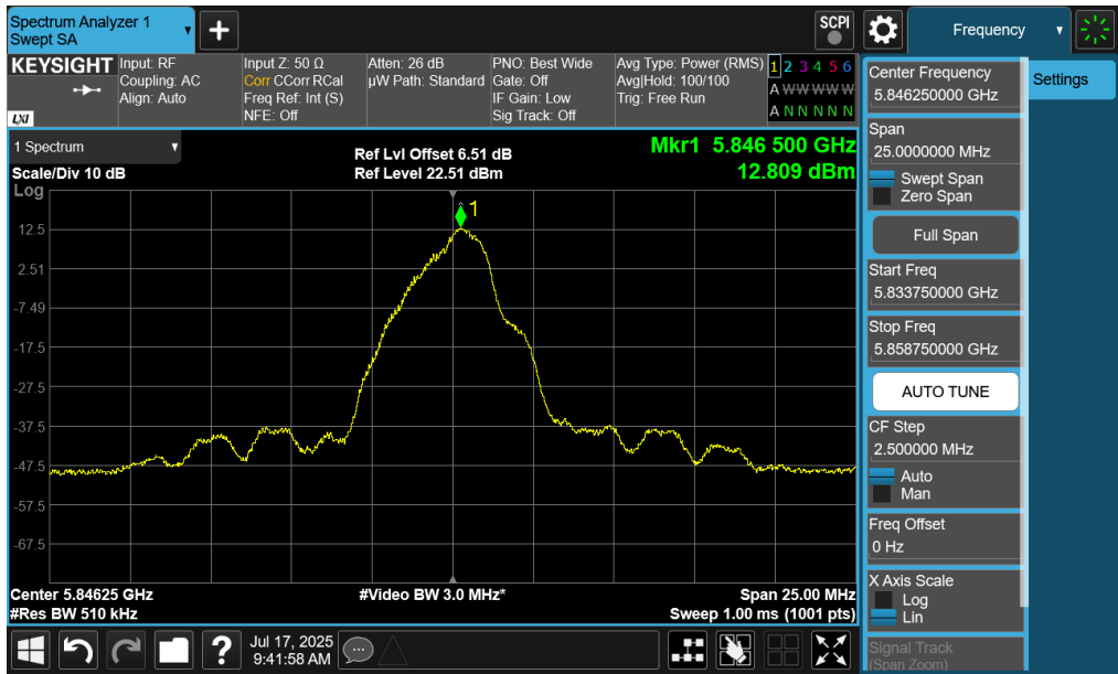
Plot 7-18. PSD (O-QPSK, 5846.25MHz, 1000kbps)
