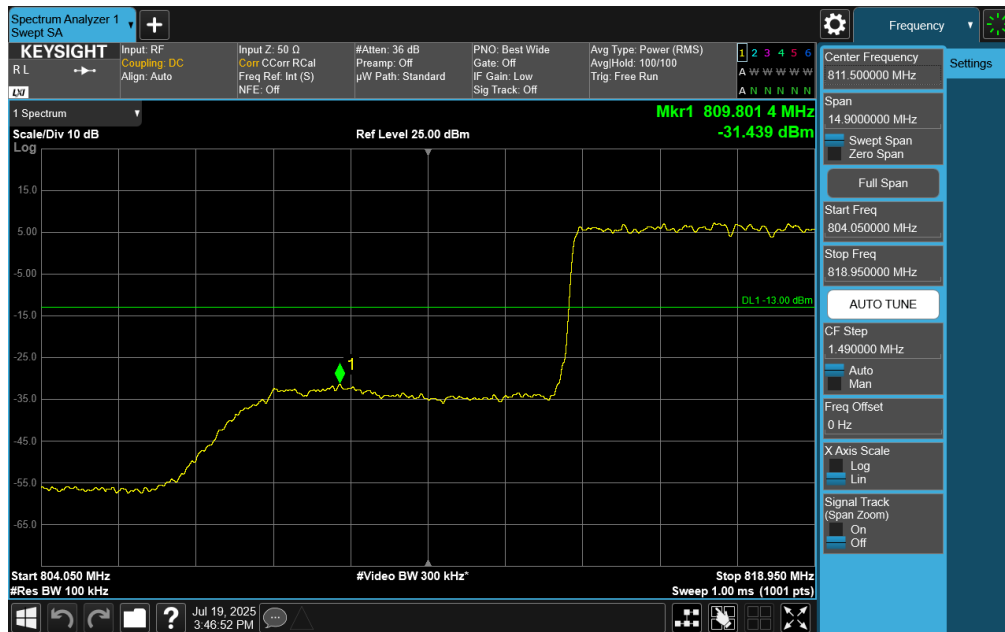
Plot 7-83. Lower Band Edge Plot (NR Band n26, 10MHz DFT-s-OFDM QPSK - RB Size 50)
