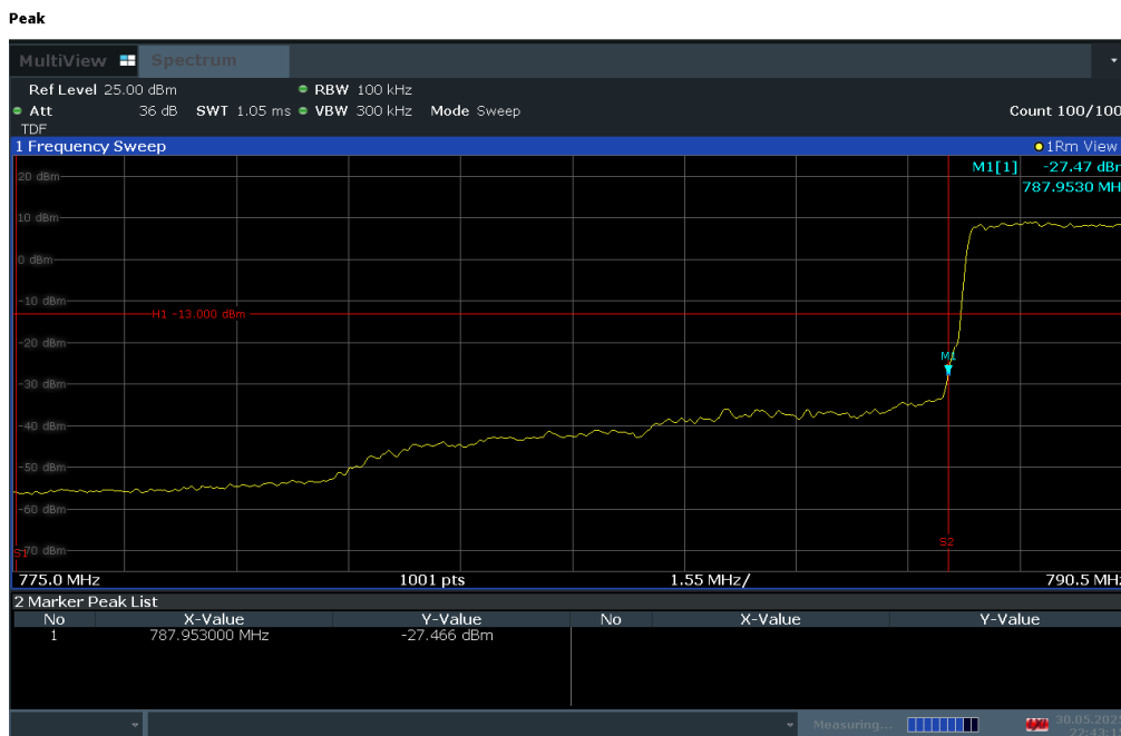
Plot 7-74. Lower Band Edge Plot (LTE Band 14, 5MHz QPSK - RB Size 25)
