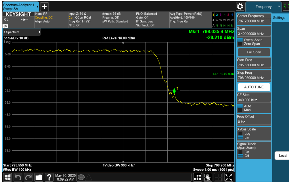
Plot 7-87. Upper Band Edge Plot (NR Band n14, 5MHz DFT-s-OFDM QPSK - RB Size 25)
