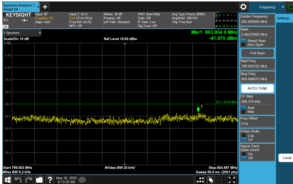
Plot 7-92. Upper Emission Mask Plot (NR Band n14, 10MHz DFT-s-OFDM QPSK - RB Size 50)
