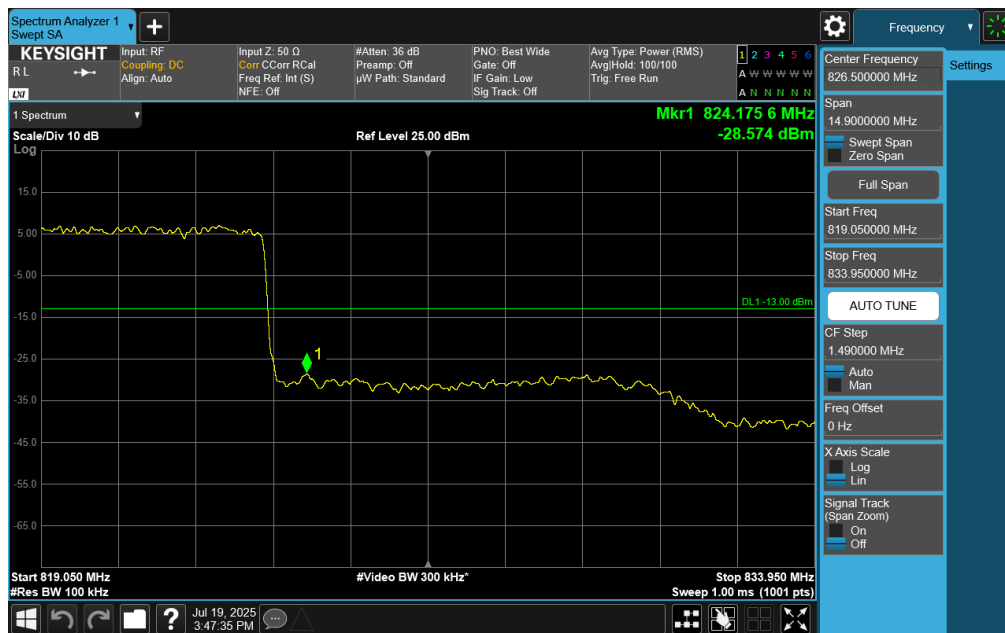
Plot 7-84. Upper Band Edge Plot (NR Band n26, 10MHz DFT-s-OFDM QPSK - RB Size 50)
