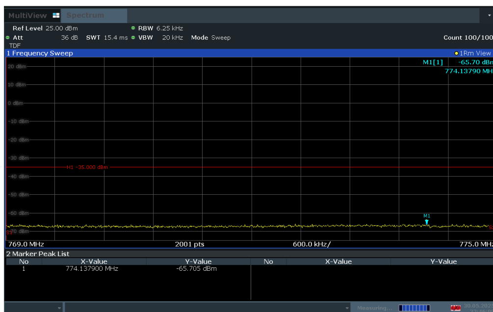
Plot 7-77. Lower Emission Mask Plot (LTE Band 14, 10MHz QPSK - RB Size 50)
