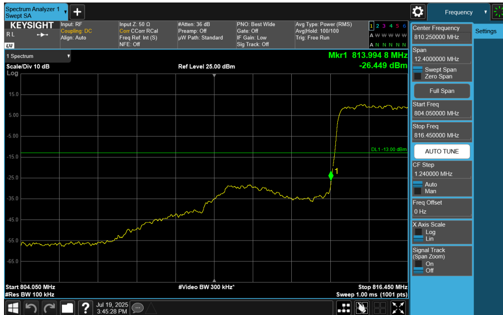
Plot 7-81. Lower Band Edge Plot (NR Band n26, 5MHz DFT-s-OFDM QPSK - RB Size 25)
