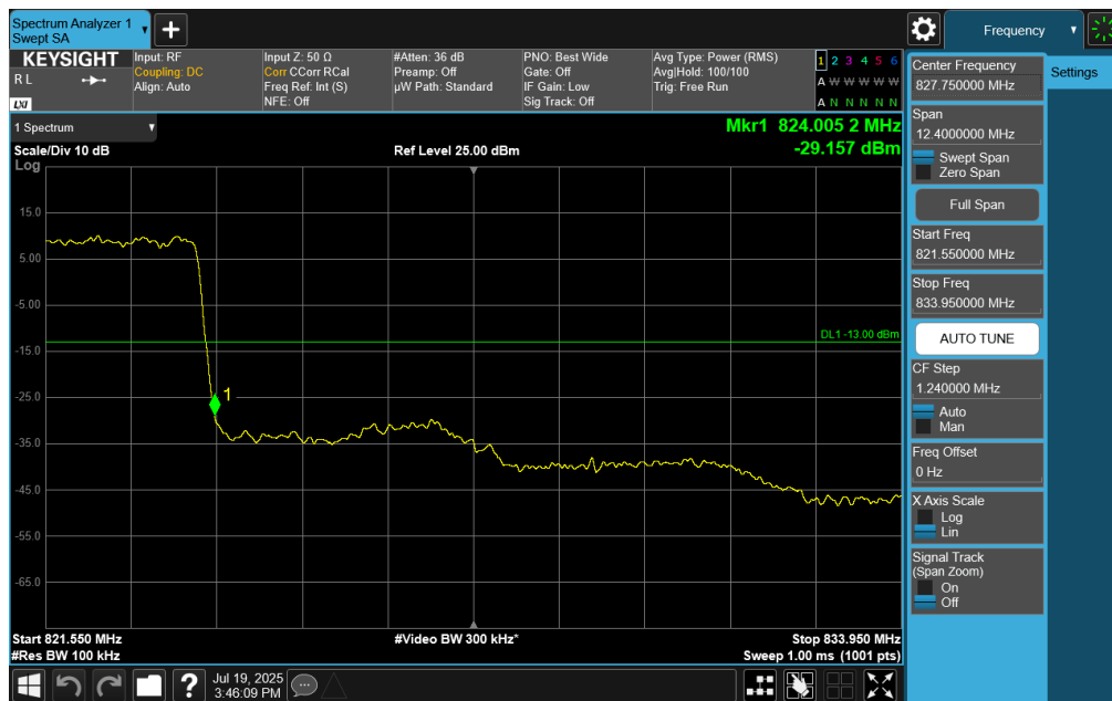
Plot 7-82. Upper Band Edge Plot (NR Band n26, 5MHz DFT-s-OFDM QPSK - RB Size 25)
