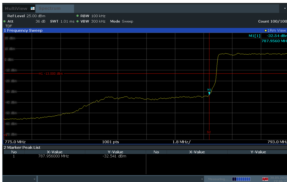
Plot 7-78. Lower Band Edge Plot (LTE Band 14, 10MHz QPSK - RB Size 50)
