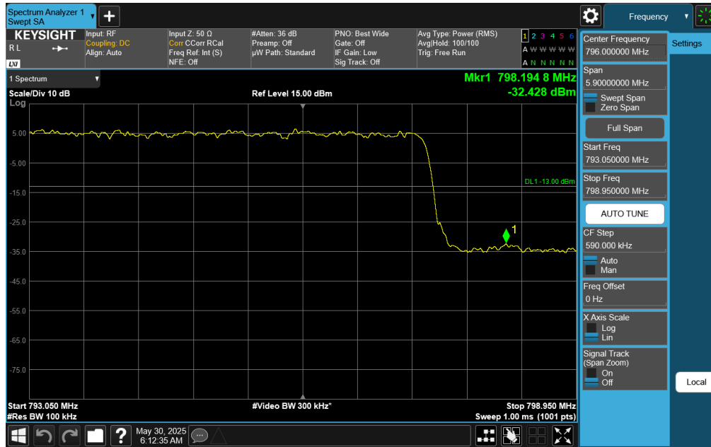
Plot 7-91. Upper Band Edge Plot (NR Band n14, 10MHz DFT-s-OFDM QPSK - RB Size 50)
