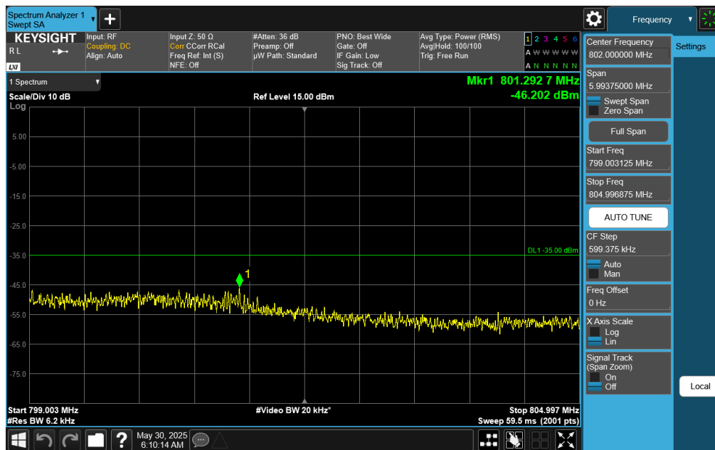
Plot 7-88. Upper Emission Mask Plot (NR Band n14, 5MHz DFT-s-OFDM QPSK - RB Size 25)
