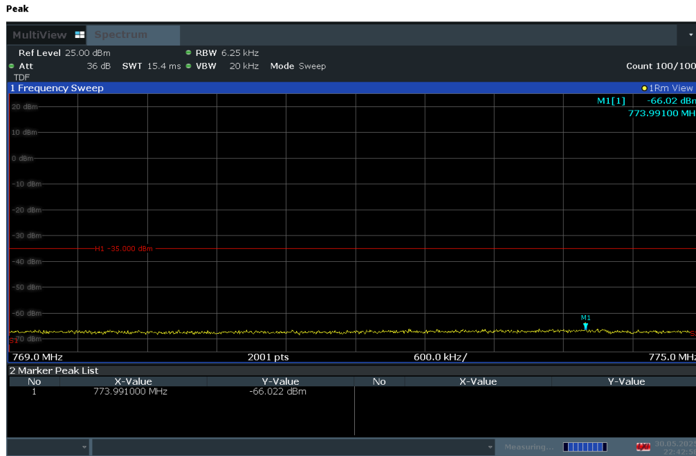
Plot 7-73. Lower Emission Mask Plot (LTE Band 14, 5MHz QPSK - RB Size 25)
