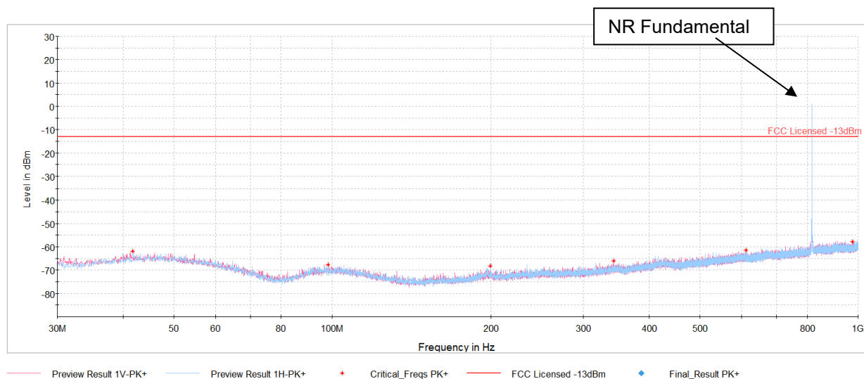
Plot 7-97. Antenna BCM Radiated Spurious Plot Below 1GHz (NR Band n26)
